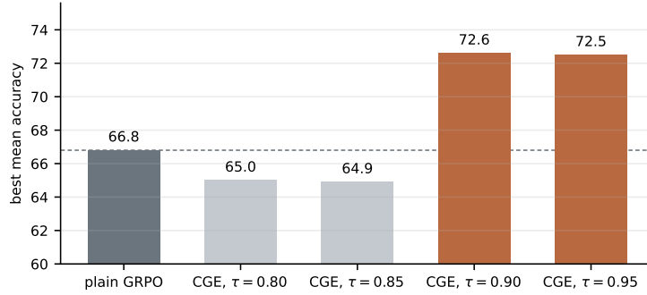
Figure 6: Best mean accuracy over the six image benchmarks of the OpenMMReasoner validation split, for plain GRPO and for CGE at four thresholds. The dashed line marks plain GRPO, and the two grey bars are the runs that never learn the answer format.
