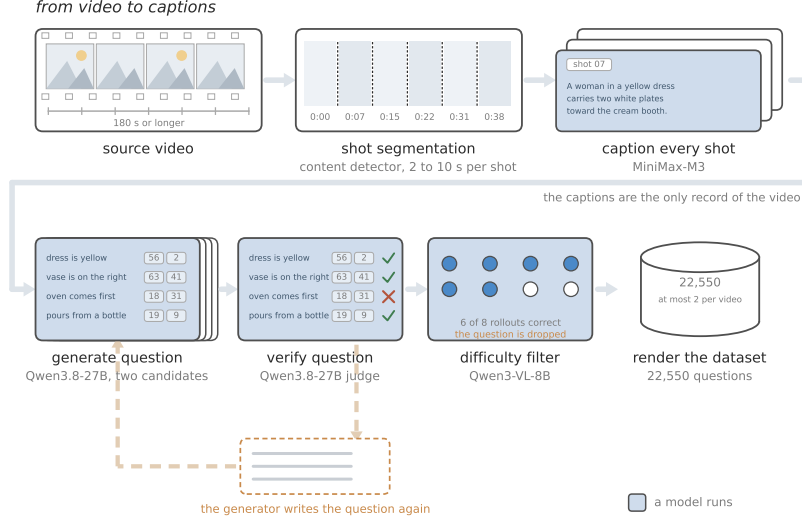
Figure 3: The Video-HopChain generator.
