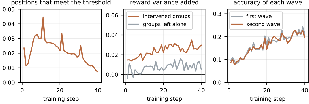
Figure 7: Three measurements of the second wave on Video-HopChain, over the training steps. The left panel gives the share of the positions the mask examines whose top-1 probability exceeds \tau , whereas the middle panel gives the reward variance the second wave adds to a group, both on the intervened groups and on the groups the mask leaves alone, which already carry variance in their first wave. The right panel then gives the training accuracy of each wave over all groups.
