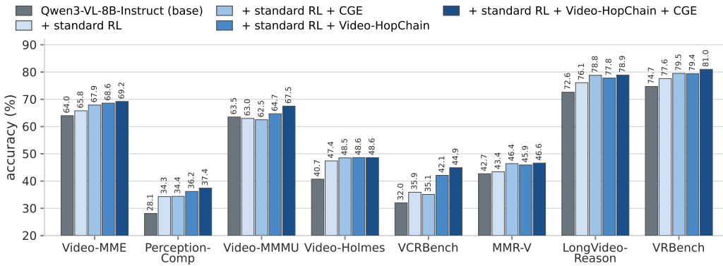
Figure 1: Main result. Accuracy on the eight public video benchmarks, for the base model and for our four training runs.
