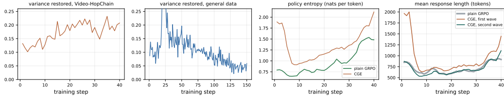
Figure 5: Four training metrics of our runs, over the training steps.
