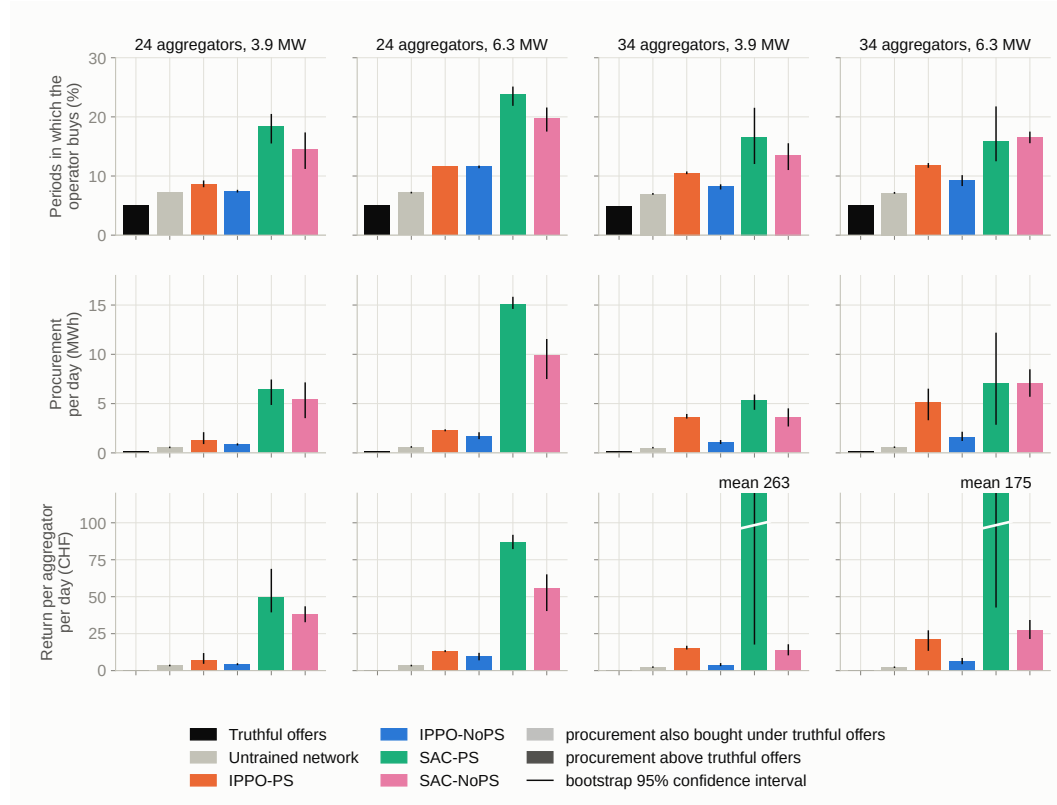
Figure 37: Source of the flexibility requirement over the 36 test days of the four configurations. Bars show truthful offers, the untrained shared and per-agent networks pooled in one bar, and the four learners at validation-selected checkpoints (seed mean and bootstrap 95% confidence interval). Two SAC-PS return bars exceed the axis and are cut at its top, with their means shown above. Rows show the share of periods with procurement; daily procurement split into what truthful offers also buy and the excess; and daily return per aggregator. Learners raise procurement above the truthful-offer level, and their returns rise with it.
