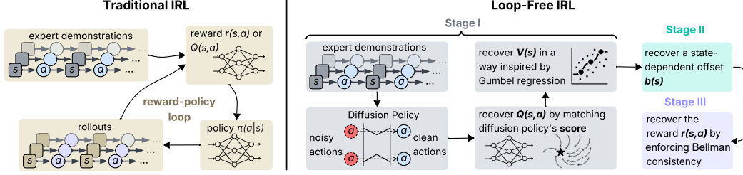
Figure 1: Traditional inverse reinforcement learning alternates between reward learning and policy optimization, while our loop-free version trains each component once without a reward-policy loop.
