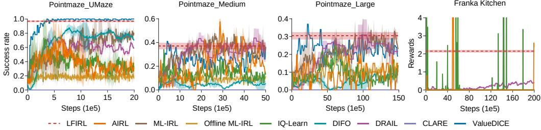
Figure 4: Reward-recovery results on PointMaze and Franka Kitchen. We report success rate on PointMaze and average completed subtasks on Franka Kitchen. Since LFIRL recovers the reward only at the final stage, its result is shown as a fixed final score rather than a policy-learning curve. For online IRL methods, “steps” denotes environment interaction steps. For offline IRL methods, “steps” denotes the number of transitions sampled from the offline dataset during training.
