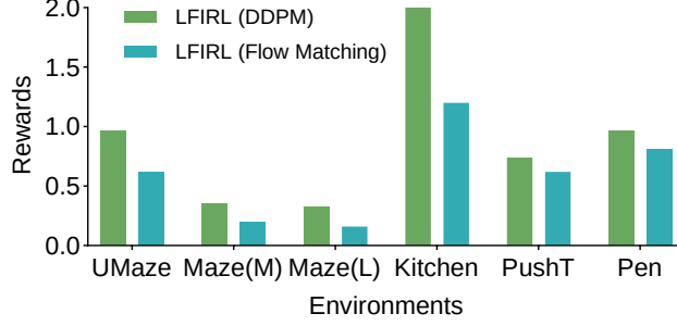
Figure 7: Additional ablation comparing DDPM-based and Flow-Matching-based pretraining in LFIRL. The two variants use the same subsequent sequential reward-recovery pipeline, but differ in how the pretrained generative policy is obtained. Higher is better.
