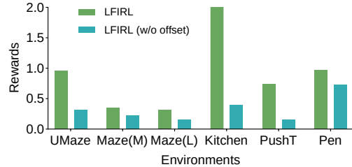
Figure 5: Ablation results on PointMaze, Kitchen, Pen, and Push-T. We compare LFIRL with its variant that removes the state-dependent offset b(s) .
