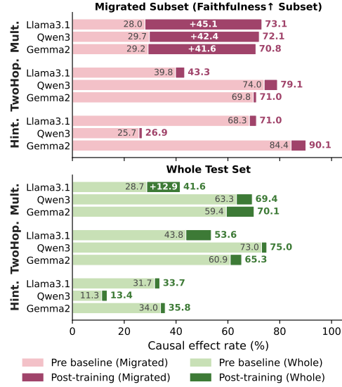
Figure 6: Causal validation of CIA improvements. Each bar shows causal effect rate on models before and after training, on both the whole test set and the migrated subset (Table 4).
