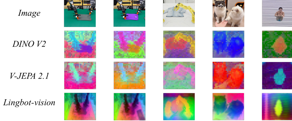
Figure 4: Qualitative comparison of frozen visual encoders on matched input images. From top to bottom, the figure shows the source images followed by response maps from DINOv2, V-JEPA 2.1, and LingBot-Vision.
