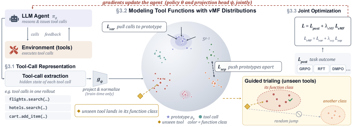
Figure 3. Overview of ToolCOMPASS. For each tool call, ToolCOMPASS extracts its final-token representation and maps it onto the unit hypersphere. Calls implementing the same function are aligned with a shared vMF prototype, while calls implementing different functions are separated. The resulting objective is optimized jointly with the post-training objective. The projection head and prototypes are not used at deployment.
