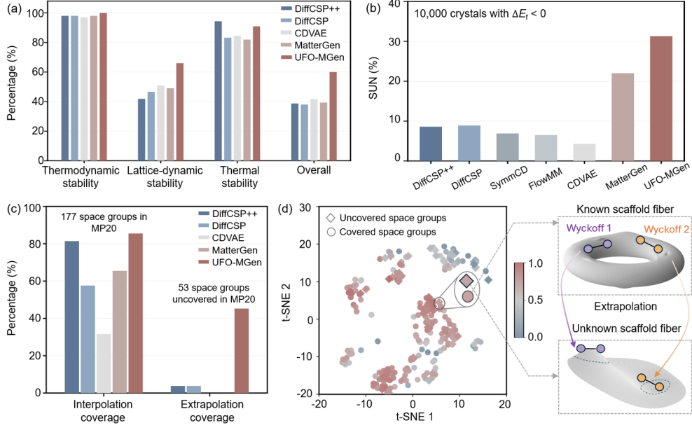
Fig. 3 Performance comparison between UFO-MGen and other generative models. (a) Comparison of the MSE success rates achieved by UFO-MGen and other generative models. (b) Comparison of the SUN rates achieved by UFO-MGen and other generative models. (c) Comparison of the interpolation and extrapolation capabilities among different generative models. (d) Similarity analysis of the scaffold features of 10,000 generated crystals visualized using t-SNE. The red color represents the high similarity and blue color means low similarity. The right schematic illustrates the extrapolation mechanism of UFO-MGen, in which crystals are generated by transferring similar Wyckoff features across neighboring scaffold fibers associated with different space groups.
