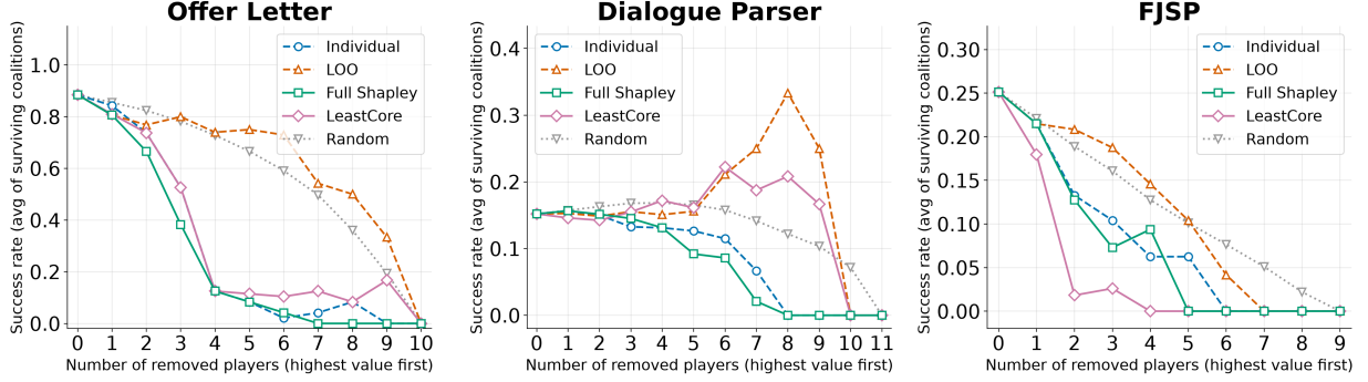
Figure 2: Experiment 1 removal validation on the three SkillsBench tasks. Each panel corresponds to one task. The x-axis is the number of removed players following each method’s ranking. The y-axis is the mean success rate over all coalitions that do not contain the removed players. Curves compare simple baselines (Individual, Leave-One-Out, and Random Removal), LeastCore [26], and full Shapley [8]. Stronger attribution should produce a sharper success-rate drop when its top-ranked players are removed.
