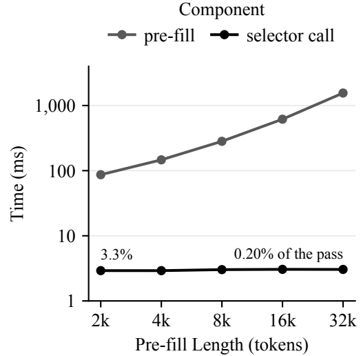
Figure 2 Selector and pre-fill latency versus input length. Measurements use Qwen2.5-7B at 4× compression, batch size 1, on one H100. The selector takes about 3 ms, or 3.3%–0.20% of pre-fill latency.
