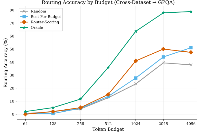
Figure 6: Router accuracy by budget level (cross-domain, GPQA). The router’s advantage is concentrated at moderate budgets ( b=512 – 2048 ), where model complementarity is highest and the oracle gap is largest.
