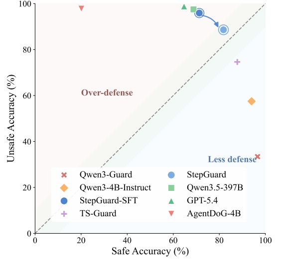
Figure 3: Safe–unsafe accuracy trade-off. Points above and below the diagonal indicate over-defense and under-defense, respectively.
