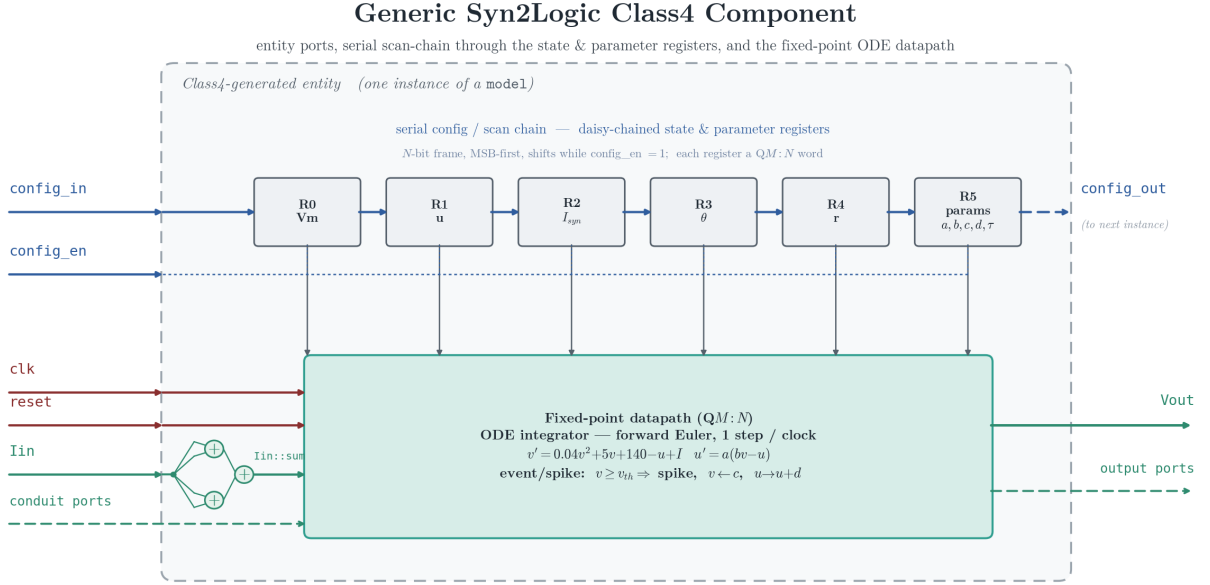
Fig. 3: A generic view of a model component generated by our Syn2Logic class4-backend. We see an Izhikevich model with several state variables, and each variable is daisy-chained on the scan-chain, which goes serially through all components in the system and can be configured from outside. The model state is connected to a generated data path that solves the ODEs and handles events. Conduits are currents from (typically connected synapses) that are added together to provide reduction functionality at the neuron side. Each conduit and output has a token (a spike-enable) signal, indicating a valid value (not entirely unlike data-flow).
