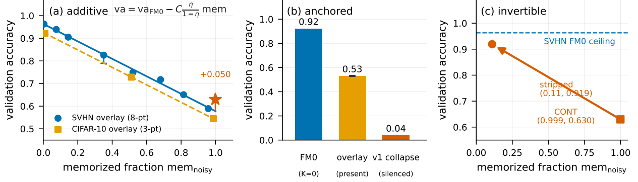
Figure 5: TLS properties. (a) Additive / billable. SVHN overlay: \text{val\_acc} vs memorized fraction, 8 points ( \text{FM0} \rightarrow K = 2500 \dots 30000 \rightarrow \text{ALL} ), with the cost-law fit va = va_{\text{FM0}} - C \frac{\eta}{1-\eta} \text{mem} drawn through them (slope -C \approx -0.386 on SVHN; CIFAR 3-point overlay in orange). K=12500 carries a real 3-seed error bar. Co-training (CONT, \star ) sits above the overlay curve at matched memory load (+0.050, SVHN resnet). The SVHN ALL endpoint shown is the ep100 checkpoint of the K=\text{ALL} run ( \text{mem } 0.958 , va 0.589); the same run’s later ep160 checkpoint ( \text{mem } 0.981 , va 0.585) saturates slightly higher but is not shown here. (b) Anchored. CIFAR three states: FM0 ( K=0 ) at 0.92, full overlay with clean present at 0.53 \pm 0.004 (3-seed), and v1 collapse with clean silenced at 0.04 — memory cannot be layered onto collapsed G . (c) Invertible. Stripping a CONT network (clean-only continuation) drains memory 0.999 \rightarrow 0.11 and recovers va 0.630 \rightarrow 0.919 , approaching the SVHN FM0 ceiling (dashed).
