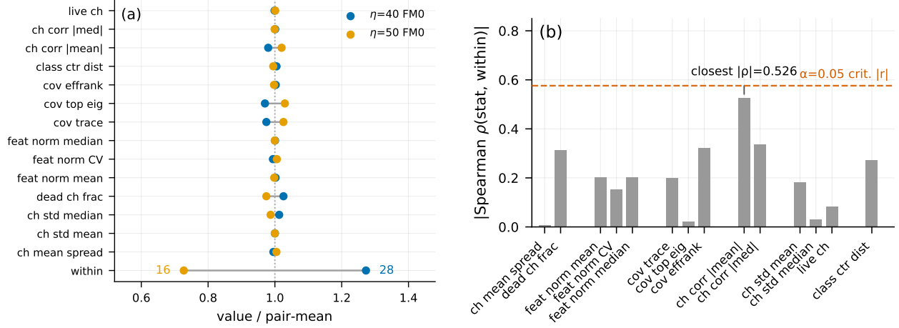
Figure 1: Instrument vindication by exclusion. (a) The decisive pairing: \eta_{40} -FM0 vs \eta_{50} -FM0, same architecture, dataset, seed and protocol. Every one of the 14 channel statistics (all normalized to pair-mean, x = 1.0 ) is near-indistinguishable between the two checkpoints ( \leq 6\% relative deviation), and \text{val\_acc} agrees to 0.3% (0.966 vs 0.963) — yet H_1^{\text{within}} differs by 12 (28 vs 16, the only row drawn with numerical labels). Two models that every global statistic treats as the same are separated by the topological readout. (b) All 14 statistics, grouped into six semantic families, plotted as |\text{Spearman } \rho(\text{stat}, \text{within})| over the 12-checkpoint CONV trajectory. None crosses the \alpha=0.05 critical value ( |r| = 0.576 , dashed red); the closest statistic is annotated once. Six families falsified.
