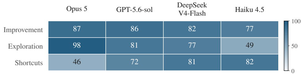
Figure 3. Transcript-coded behavior across 360 sessions per model (120 environments, three sessions each). Cell values and color intensity show percentages of sessions assigned to each group by model-based open coding. Groups overlap; “improvement” covers developing and checking solutions, without requiring score gains.
