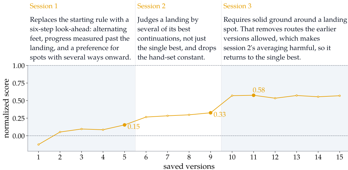
Figure 4. A three-session Claude Opus 5 chain on a foothold-selection task. Open points are saved solutions graded on the held-out test set; filled points mark final submissions, with normalized scores of 0.15, 0.33, and 0.58. The annotations summarize the changes recorded in each session. The third session adds a ground-support check and reverses the second session’s averaging rule.
