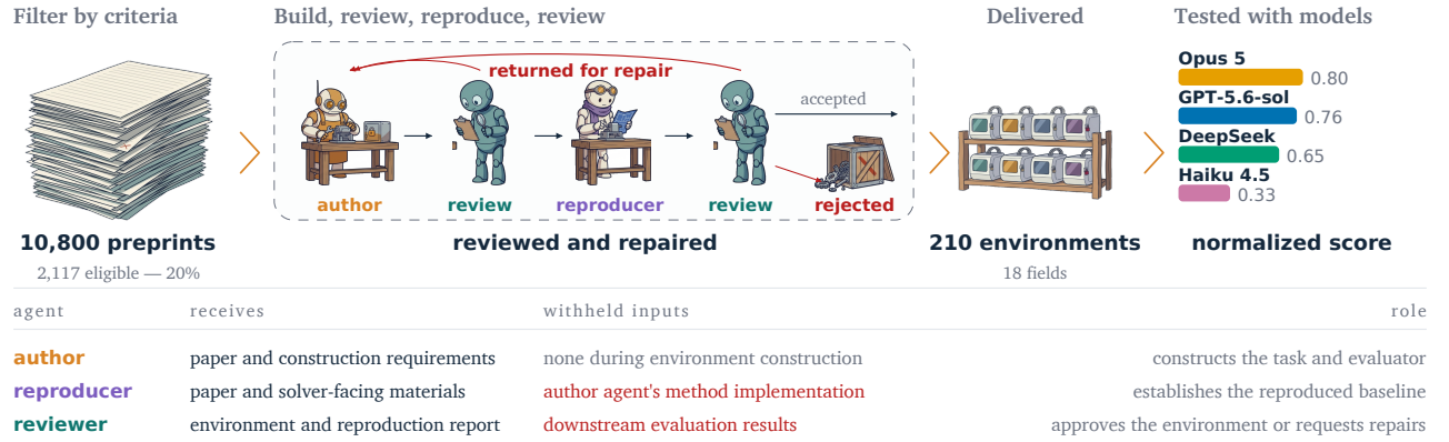
Figure 1. Overview of RSI-Forge and the information available to each agent. Failed checks lead to repair or rejection before an environment is accepted. The output count includes all 210 environments. The performance bars report median scores of final solutions after 3 successive attempts on 120 environments sampled from the main construction run. Scores are normalized so that the starting solution is 0 and the target score is 1 (Eq. (1)).
