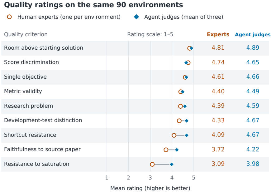
Figure 2. Quality ratings from human experts and agent judges on the same 90 environments, with one expert and three judges per environment. Points show means on a 1–5 scale (higher is better). Agent ratings are averaged within environments; rows are ordered by expert mean. Only experts received available solver results. Appendix B.2.2 and Table 6 give the rubric and per-dimension standard deviations.
