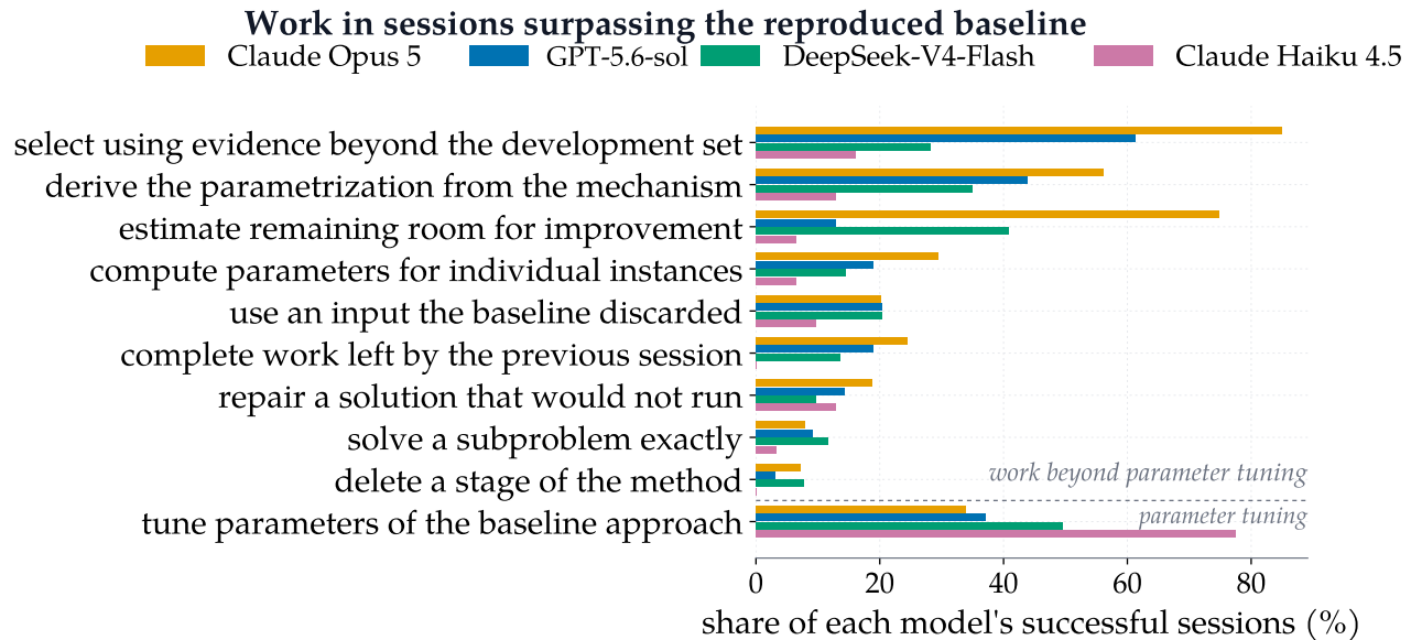
Figure 5. Transcript-coded mechanisms as percentages of each model's sessions that surpass the reproduced baseline. The codebook was derived from a sample and fixed before counting. Sessions may receive several labels; nine categories cover work beyond parameter tuning. The labels describe work within the constructed task and do not establish scientific novelty.
