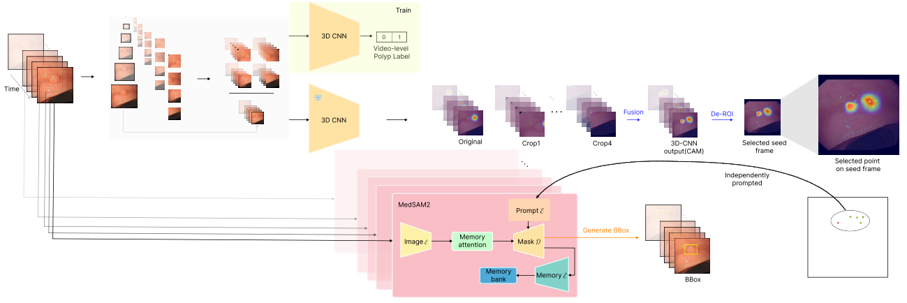
Fig. 1: Overall framework of the proposed method. Given an input video clip, a 3D CNN predicts video-level polyp presence and generates class activation maps (CAMs), from which candidate points are derived. Each point is independently provided to MedSAM2 as a prompt, which propagates the resulting mask across the clip to produce the final localization.
