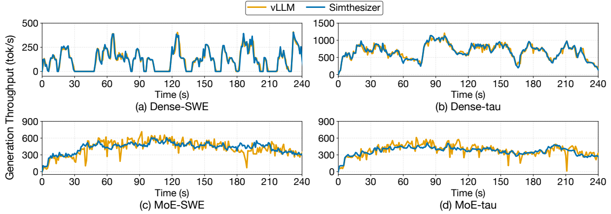
Fig. 8. Comparison of throughput between unmodified Synthesizer (without any agent-synthesized extension) and a GPU-based serving system running vLLM under agentic workloads: (a) Llama3.1 dense model on mini-SWE-bench, (b) Llama3.1 dense model on tau-bench, (c) Qwen3 MoE model on mini-SWE-bench, and (d) Qwen3 MoE model on tau-bench.
