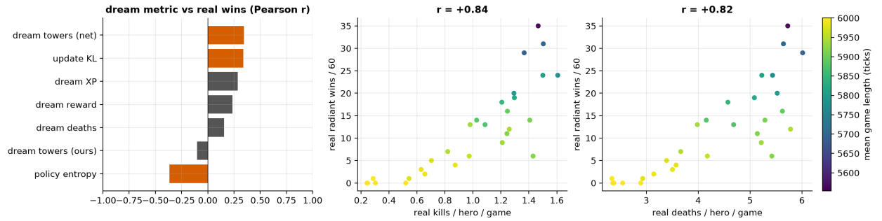
Figure 4: During a collapse, nothing measured in the dream tracks real wins (left), while the policy’s real behaviour does: real kills (middle) and deaths (right) per hero and game against real wins, coloured by game length.
