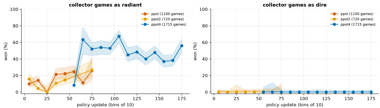
Figure 9: The collector’s real games, binned by policy update: an independent stream of real performance on fresh seeds. The anchored run (blue) holds 45–67% as radiant where the unanchored runs held 0–27%, and shows a late dip that the drift guard did not catch.
