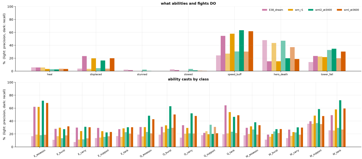
Figure 8: World-model fidelity per mechanic on the policy’s own games, for each world-model version (light: precision, dark: recall).
