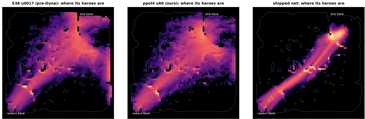
Figure 6: Where the radiant heroes spend their time, over 20 games each: the pre-loop policy (left), the final policy (middle) and the shipped net (right). The net moves as one group down the middle lane; both dream-trained policies cover the whole map.
