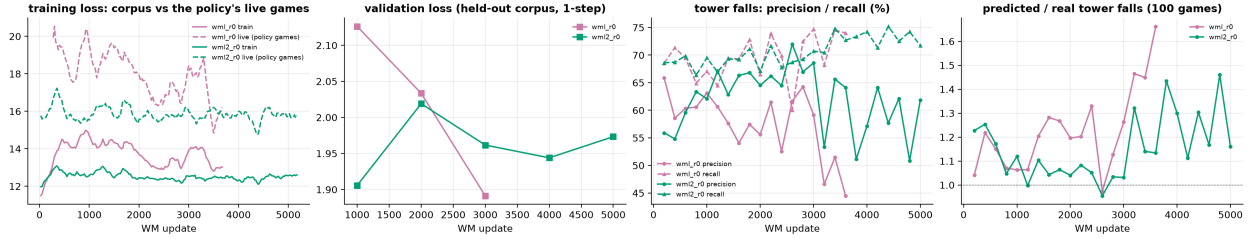
Figure 10: The world model during the loop: training loss on the corpus and on the policy’s newest games, held-out validation loss, and tower fidelity per checkpoint.
