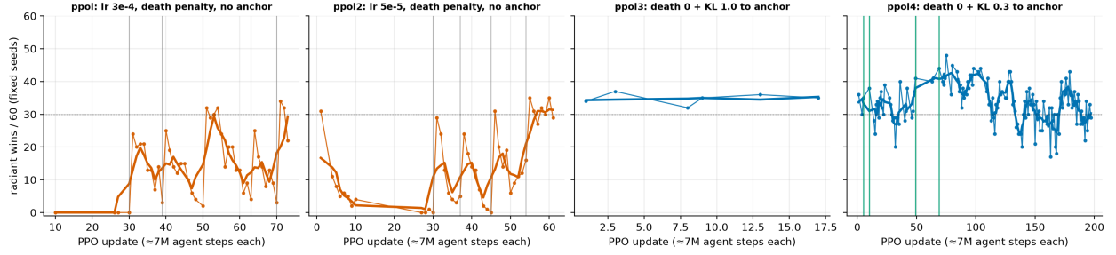
Figure 3: Real radiant wins out of 60 after every PPO update. Without an anchor the policy collapses repeatedly (grey lines: drift resets); with the death penalty removed and a KL anchor it holds and improves (green lines: a new anchor confirmed on fresh seeds).
