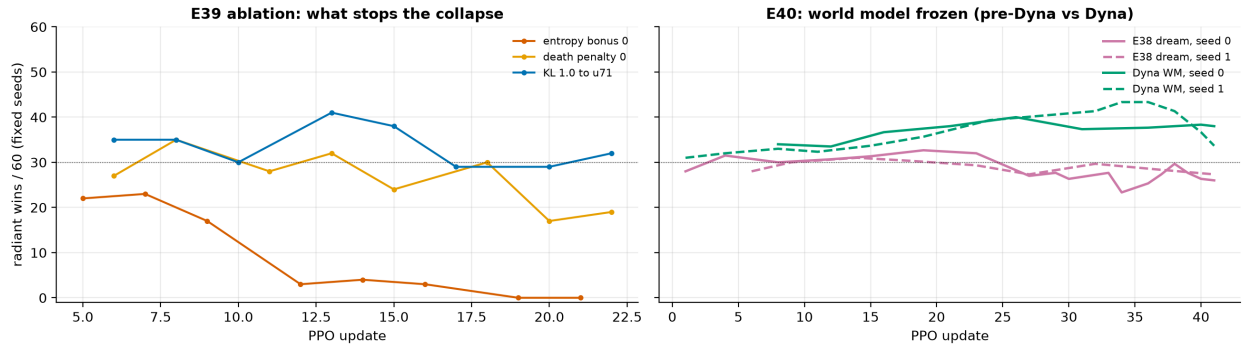
Figure 11: Left: what stops the collapse (one seed per arm). Right: the frozen-world-model control, real wins during training.
