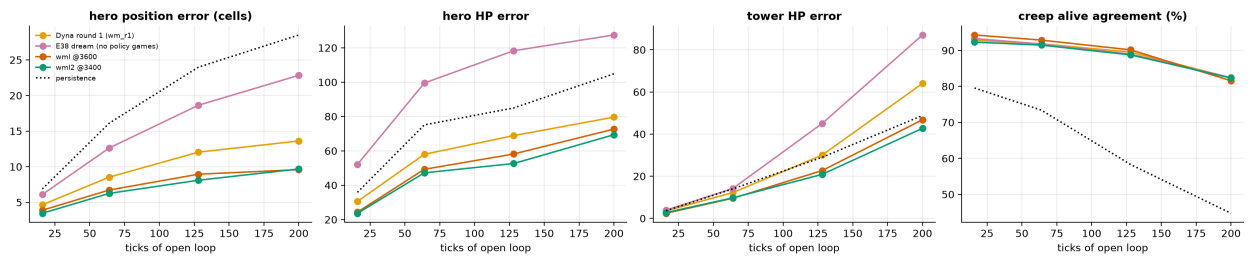
Figure 5: Open-loop divergence from the real game on the policy’s own games, by horizon. The pre-Dyna model (pink) is worse than predicting no change (dotted) for hero and tower health; the Dyna models are better at every horizon.
