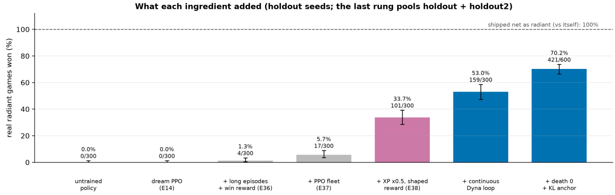
Figure 7: The contribution ladder on the holdout seeds, with 95% Wilson intervals.
