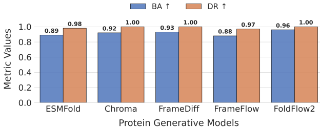
Figure 10: MARCO vs. Refolding . By selectively altering the translated sequences, MARCO gains sufficient robustness against refolding attack.
