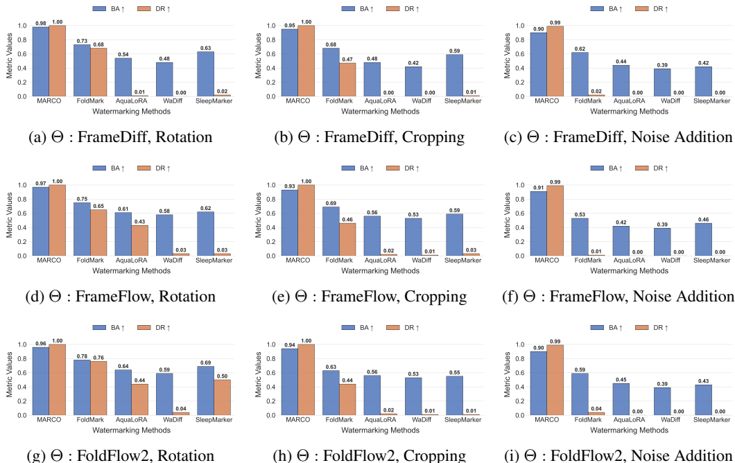
Figure 6: Part B – Evaluation of Robustness of PGM Watermarking Methods against Conformation Manipulations . After conformation manipulations, MARCO survives and outperforms the other four baselines with impressive robustness.
