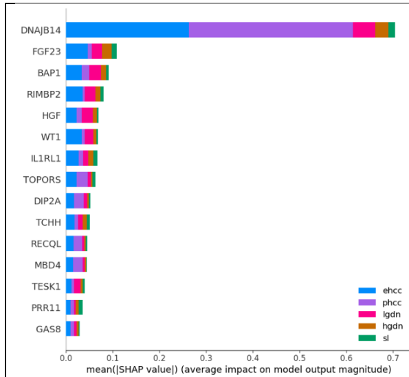
Figure 8 PSO Graph
