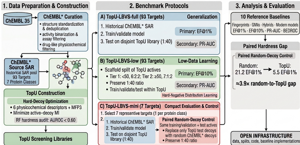
Figure 1: TopU-LBVS framework . ChEMBL 35 is curated into ChEMBL*, which supplies historical SAR data and the inactive pool for constructing TopU hard-negative libraries. TopU-LBVS-full evaluates generalization from historical ChEMBL* SAR to disjoint TopU screening libraries; TopU-LBVS-low evaluates learning from limited labeled data within the TopU hard-negative distribution; and TopU-LBVS-mini provides a seven-target protocol with a paired random-decoy control that changes only the test decoys.
