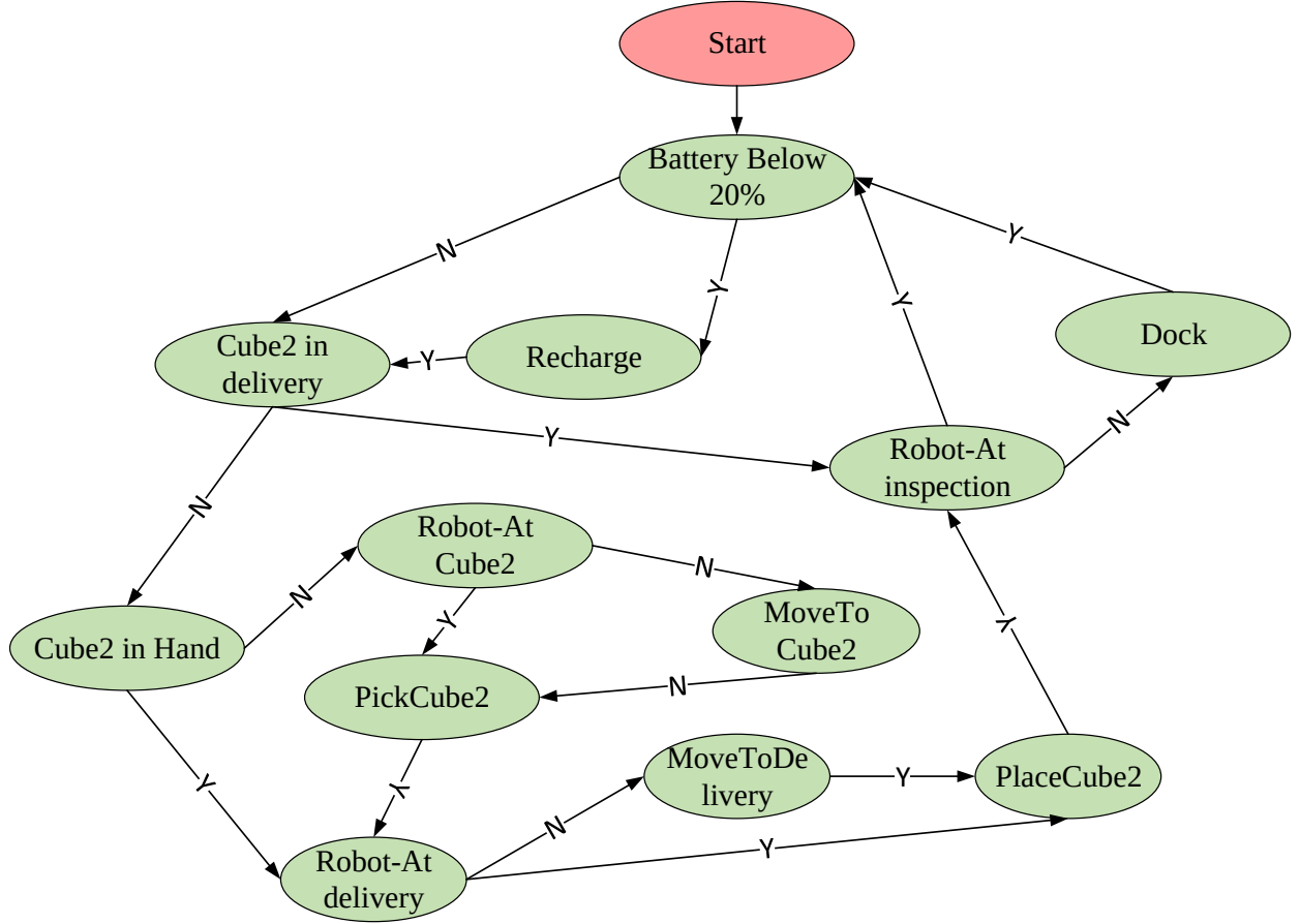
Figure 17: FSM generated by NLLM.
