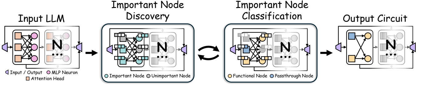
Figure 2: An overview of the proposed S³martCirc framework.
