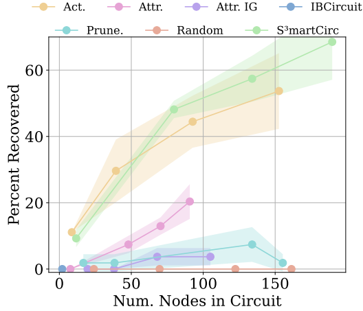
Figure 3: Percent of the IOI circuit recovered by different circuit discovery methods
