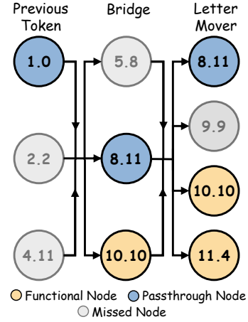
Figure 4: Comparison between the Acronym circuit and the functional interpretations determined by S³martCirc.
