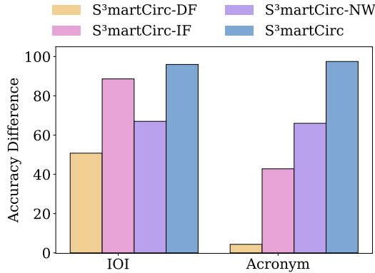
Figure 6: Ablation study to evaluate the effectiveness of different components in S^3\text{martCirc} and its training process.
