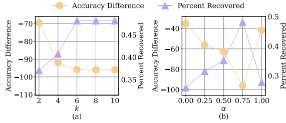
Figure 5: Effect of \alpha and k on S^3\text{martCirc} Performance.
