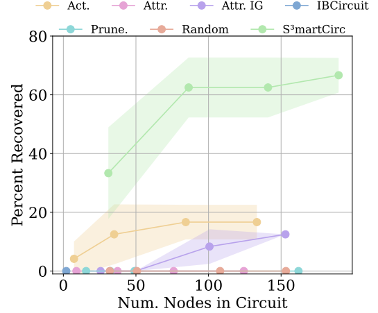
Figure 7: Percentage of the Acronym circuit recovered by different circuit discovery methods
