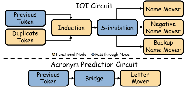
Figure 1: Mapping between node-specific functional roles in discovered circuits and the defined general functional roles.
