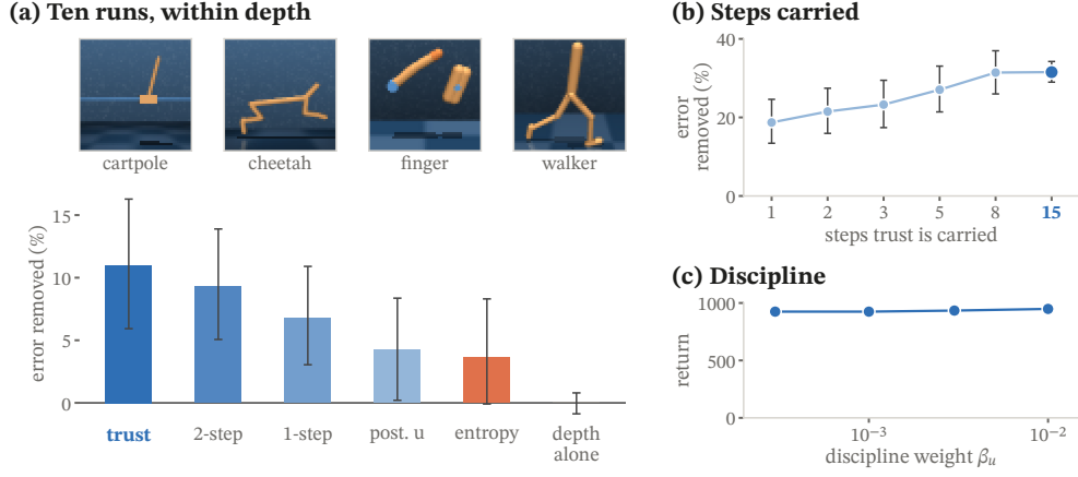
Figure 20: Trust across ten runs, and two hyperparameters. (a) Error removed by dropping the worst fifth of imagined steps, ranked within each depth as in the solid bars of Fig. 7, averaged over ten runs across walker, cheetah, finger and cartpole; top: the four tasks. (b) The same, ranked over all depths on cheetah from pixels as in Fig. 7b, with trust compounded over the last w steps; w = 15 : the whole rollout, as in LucidWM. (c) Return on walker against the discipline weight \beta_u . Whiskers: bootstrap 95% intervals.
