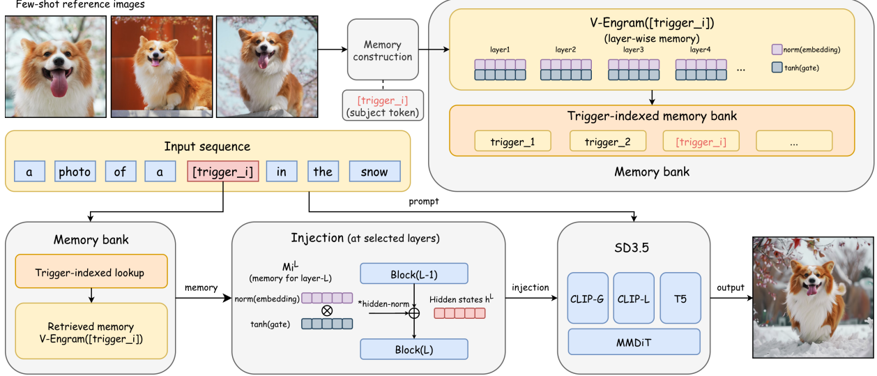
Figure 2: Overview of V-Engram. Few-shot references and an explicit trigger construct tokenizer-specific, layer-wise Engram entries. Exact token-id matches retrieve entries whose residuals are injected into selected frozen Stable Diffusion 3.5 layers.
