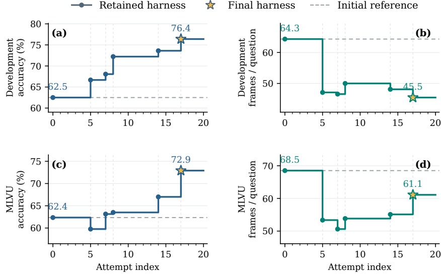
Figure 3: Evolution over 20 revision attempts. Accuracy and mean frames per question on (a,b) the development set and (c,d) MLVU. Curves track the retained harness. Vertical guides mark accepted revisions, and flat intervals indicate an unchanged incumbent.
