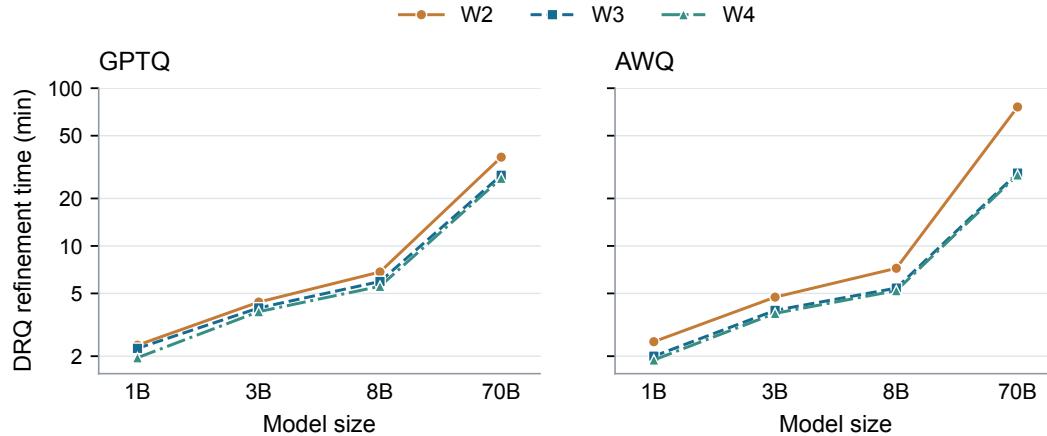
Figure 8: DRQ refinement time across model sizes and weight bit widths.
