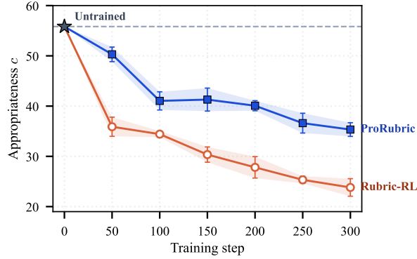
Figure 5: Appropriateness during training. Medical 4B, 300 HealthBench-consensus prompts; three-seed mean \pm standard deviation, step 0 is the untrained model.
