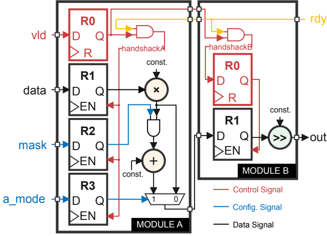
Fig. 2. A typical single-stage synchronous circuit design for analyzing the source of dynamic power.
