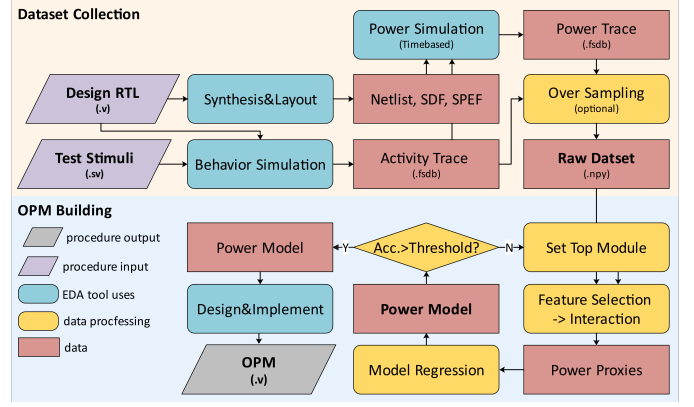
Fig. 4. The proposed automatic modeling pipeline
