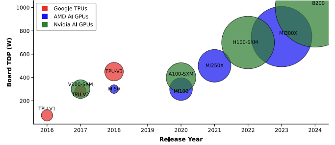
Fig. 1. Board TDP (Thermal Design Power) versus release year of recent cloud AI processors.
