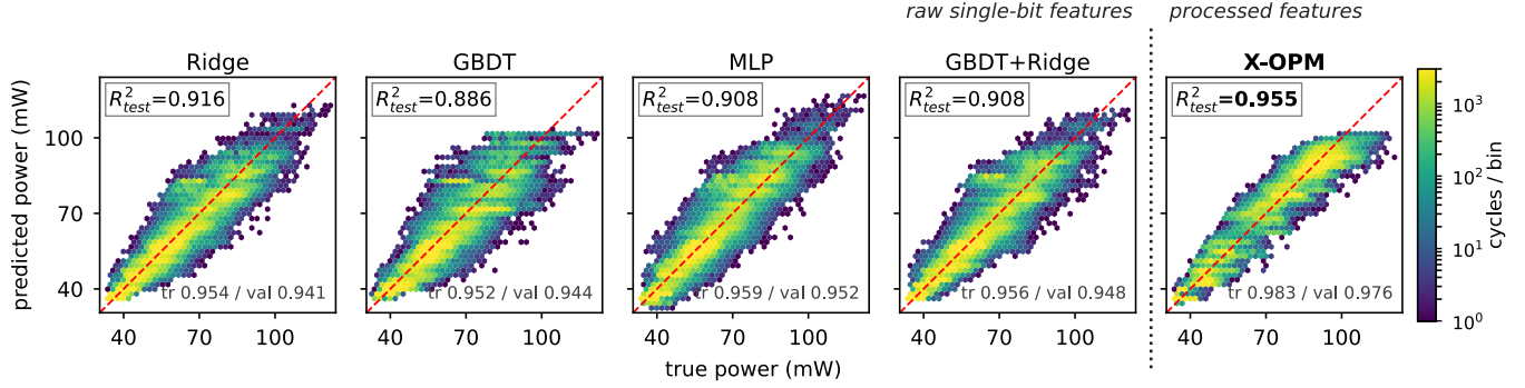
Fig. 7. The residual plot shows the predicted versus true per-cycle power of x_aq_core on the test benchmarks. The four baselines on the left are trained on raw single-bit features; X-OPM is trained on the processed features. Each hexagon bin is colored by the number of cycles it holds; the red dashed line marks perfect prediction. Train and validation R^2 are listed in the lower-right corner of each panel.
