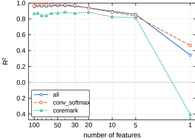
Fig. 8. Test R^2 of the C906 OPM versus the number of retained proxies under RFE pruning.
