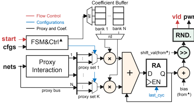
Fig. 5. Architecture of the OPM predictor and its model evaluation datapath.
