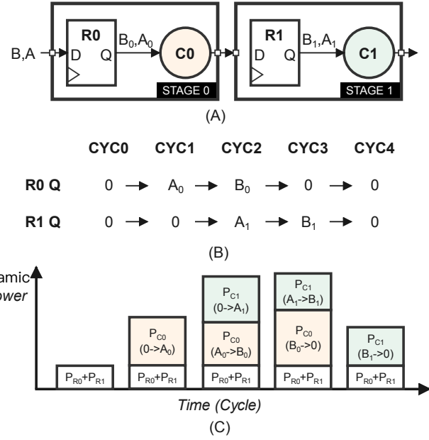
Fig. 3. Dynamic power fluctuation of a two-stage pipeline. (A) Block Diagram of the pipeline (B) Data toggle at the output of two registers. (C) Per-cycle dynamic power decomposition.
