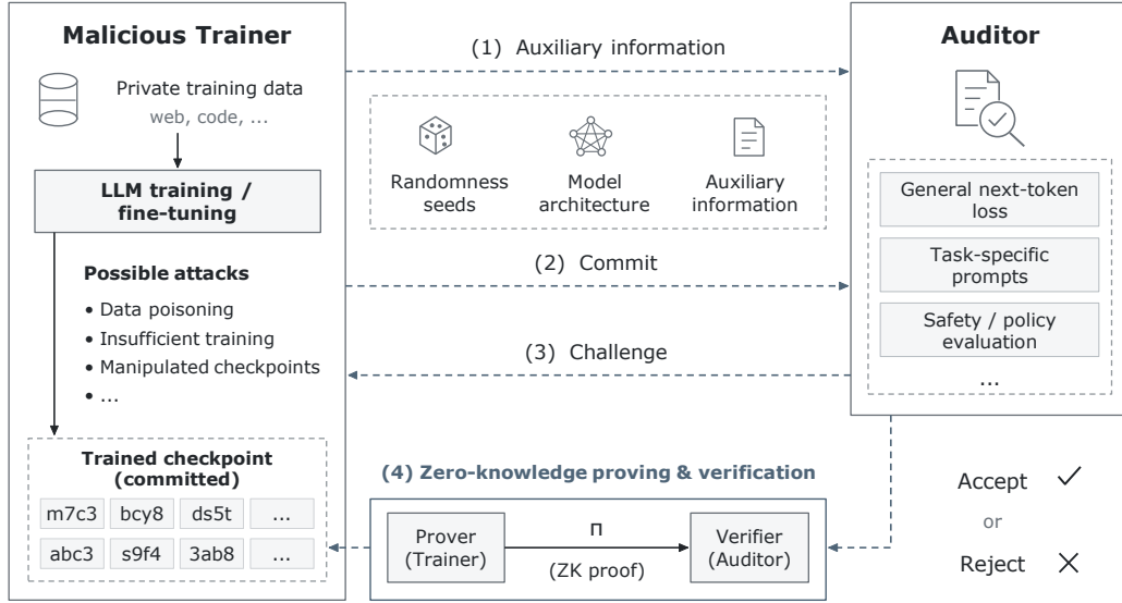
Figure 1: Audit workflow of zkLLMPoT. After publishing public auxiliary information, the trainer commits a checkpoint. The auditor then issues challenge sequences under a chosen objective (next-token loss, task prompts, or a safety check). The auditor verifies a zero-knowledge proof and accepts or rejects the claimed outcome without learning the private training data or model weights.
