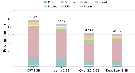
Figure 2: Per-operator proving time at T=512 for the four 1.xB checkpoints of Table 1.
