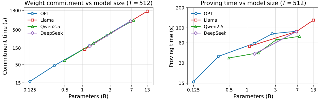
Figure 3: Dense-weight commitment and covered proving cost against model size at T=512 . Every linear shape was measured directly on the A100. Nonlinear argument costs are interpolated from measured size curves, and their opening-preparation costs are fitted from measured openings.
