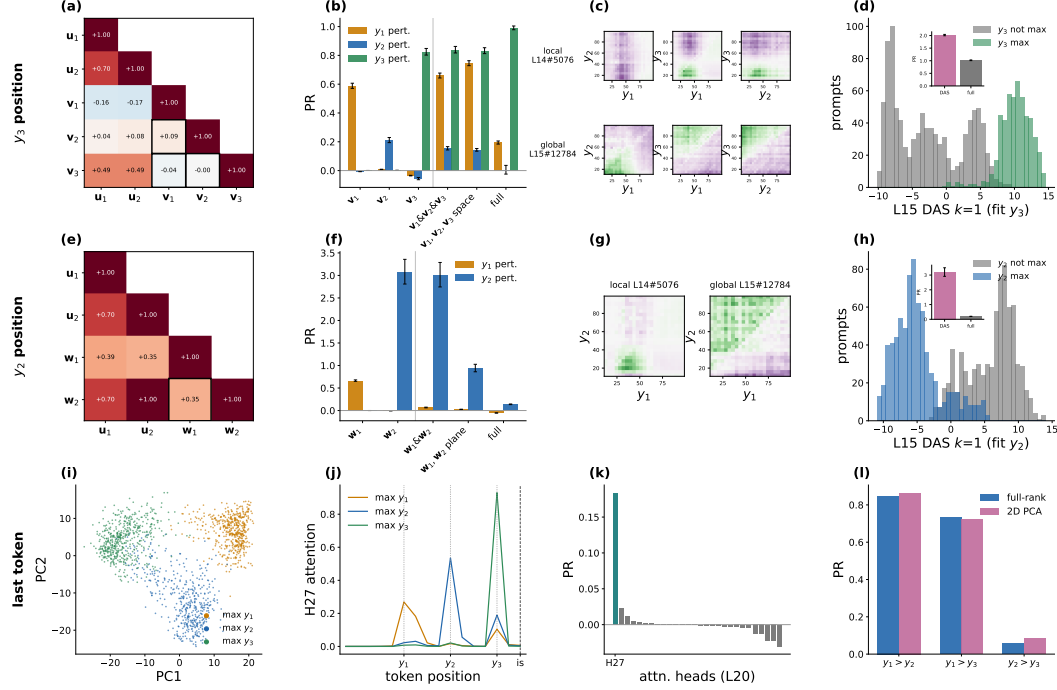
Figure 26: The three-number analysis at the position of y_3 (top row), the position of y_2 (middle row) and the last token (bottom row). (a) Cosine similarities between u_1, u_2, v_1, v_2 and v_3 ; the pairs among v_1, v_2, v_3 are boxed. (b) Position recovery at the position of y_3 , by perturbed number, for each direction alone, the three as separate rank-one patches, their span in the pre-MLP layer-14 residual, and the full layer-14 residual. (c) Receptive fields of L14#5076 (top) and L15#12784 (bottom) at the position of y_3 over a (y_1, y_2, y_3) grid with stride 4, shown as the three pairwise marginals, each averaged over the third number and divided by its own peak. (d) The 1,500-prompt cloud projected on a rank-one direction in the layer-15 residual fitted with y_3 perturbed, split by whether y_3 is the maximum; the inset shows the position recovery of this direction and of the full layer-15 residual. (e–h) The same at the position of y_2 , where w_1 and w_2 are rank-one directions in the layer-13 residual fitted with y_1 and y_2 perturbed ( w_2 and u_2 are the same fit). The fields in (g) are over (y_1, y_2) with y_3 = 55 . (i) Top two principal components of the residual leaving layer 20 at the last token, coloured by which operand holds the maximum. (j) Attention of head L20.H27 from the last token to the question tokens, averaged by the position of the maximum. (k) Position recovery of each layer-20 head’s own output at the last token, for the order y_1 > y_2 > y_3 . (l) Position recovery of a full-rank patch and of a patch of the top two principal components of the layer-20 residual at the last token, for three value orders; the principal components are fitted on a separate 1,500-prompt cloud.
