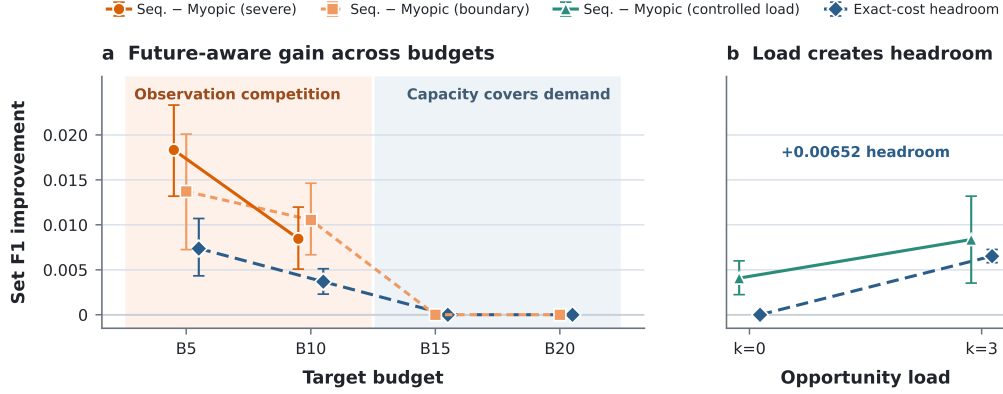
Figure 2: Future-aware gains follow the demand–capacity boundary. a: Sequential-minus-Myopic Set F1 gains on two disjoint tests and exact-cost structural headroom are positive at B5/B10, where observations compete, and zero at B15/B20, where capacity covers demand. b: At fixed B10, the controlled-load test shows that increasing opportunity load creates 0.00652 exact-cost headroom while Sequential remains above Myopic. Error bars show paired-bootstrap 95% CIs.
