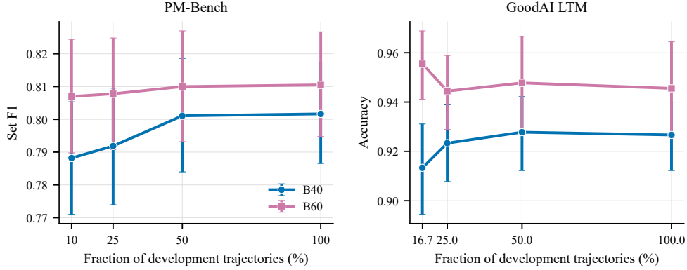
Figure 3: Held-out quality versus Outcome-label data. Error bars are paired bootstrap 95% CIs over analysis seeds 4000–4029. GoodAI reaches an early performance plateau.
