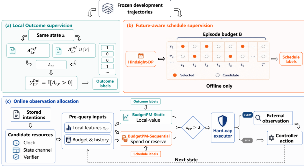
Figure 1: Overview of BudgetPM. Frozen development trajectories provide cached observation results for constructing (a) local Outcome labels and (b) hindsight-DP schedule labels under an episode budget. At deployment (c), Static or Sequential uses only pre-query inputs; thresholded proposals pass through a shared hard-cap executor that enforces the per-step and episode limits. Future information is used only for offline supervision.
