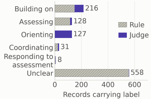
Figure 4: Multi-agent analysis of one TabPFN epoch. A: activity across 131 agent sessions and four shared-file tracks in source-log order. Arcs connect earlier writes (open symbols) to later cross-agent reads (filled symbols); colour and shape denote context type. B: all 922 access records by resource path. C: inferred purposes, with compound labels counted in each category. Access does not establish uptake.
