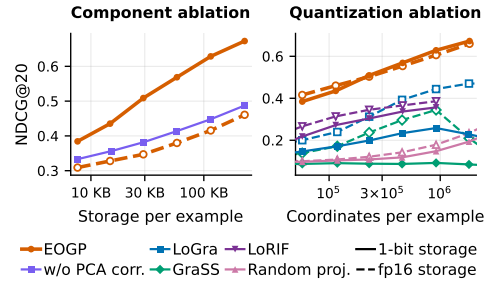
Figure 5: Component ablation of EOGP (left) and comparison of 16-bit and 1-bit storage at matched coordinate counts (right).
