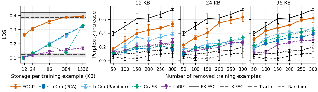
Figure 2: Validation against retraining-based ground truth on GPT-2 across storage budgets: linear datamodeling score (left) and counterfactual retraining (right). Black lines denote uncompressed influence functions with different Hessian approximations and the random-removal baseline.
