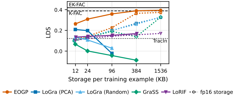
Figure 7: LDS of compression methods under one-bit and FP16 storage on GPT-2 at matched per-example storage budgets. Horizontal lines denote uncompressed references. Curves end where the required projection dimension exceeds the method’s supported dimension.
