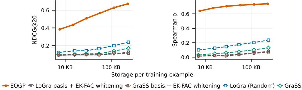
Figure 6: Comparison of EOGP with LoGra and GraSS on OLMo 2 7B SFT, using either their original curvature treatment or EK-FAC half-whitening before projection. NDCG@20 (left) and Spearman correlation (right) measure agreement with EK-FAC influence at matched per-example storage budgets.
