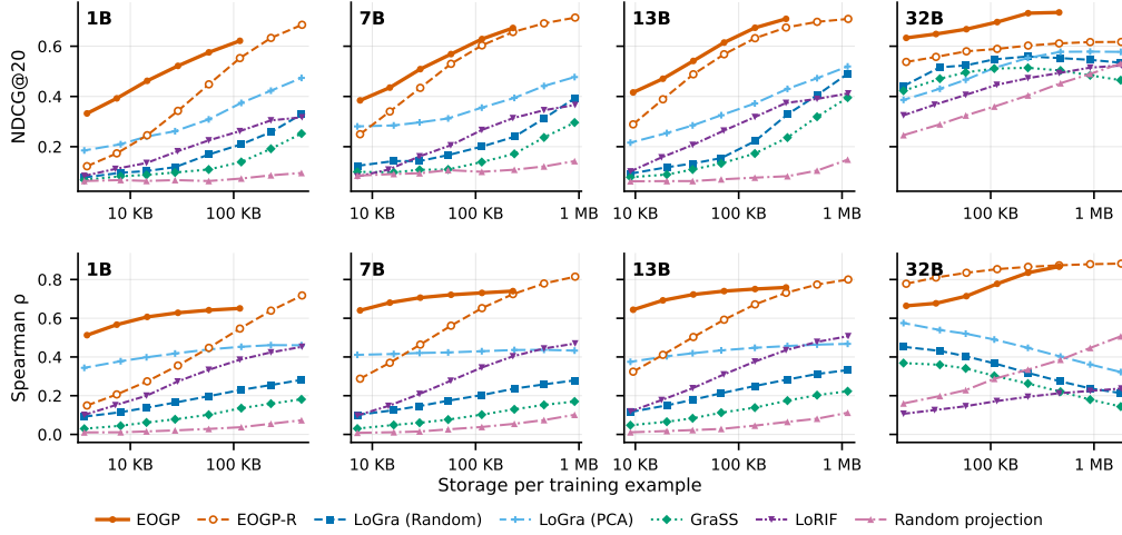
Figure 4: NDCG@20 (top) and Spearman correlation (bottom) of gradient compression methods against EK-FAC influence functions on OLMo 2 SFT models from 1B to 32B parameters.
