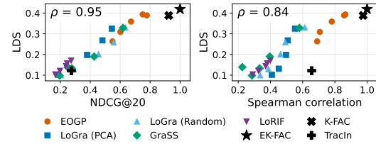
Figure 3: LDS versus EK-FAC fidelity on GPT-2, measured by NDCG@20 (left) and Spearman correlation (right). \rho is the Spearman correlation across configurations from Figure 2.
