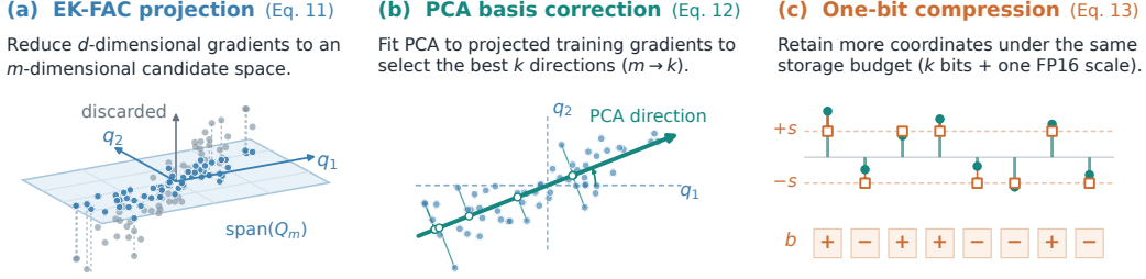
Figure 1: Overview of EOGP. (a) Training gradients are projected onto an EK-FAC subspace and half-whitened. (b) PCA corrects the compression basis within this subspace. (c) The resulting coordinates are stored as one sign bit per coordinate together with a shared scale. Query gradients undergo the same transformations without one-bit quantization, and influence scores are computed as scaled inner products with the stored bits.
