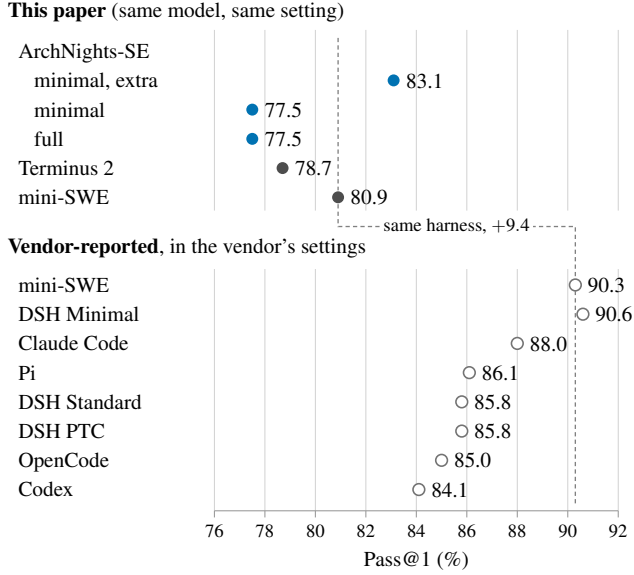
Figure 8: Terminal-Bench 2.1, Pass@1 by harness, with deepseek-v4.1-flash as the Oracle. This paper (filled dots, ArchNights-SE in blue, in the configurations of Table 9): one trial of each of the 89 tasks, with the same model in the same setting. Minimal, extra: the minimal system with the extra prompt; otherwise the minimal and the full system use the default prompt. Vendor (hollow dots): as reported in [101], Table 4, in the settings given there. In each group the dashed line marks the score of mini-swe-agent, the harness both evaluations run, and it joins the two scores. mini-SWE is mini-swe-agent, and DSH is DeepSeek Harness.
