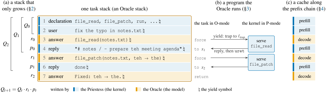
Figure 1: One history, three readings. A session in which an agent fixes a typo, as the records of one task stack. The Priestess (the kernel) writes the blue records and the Oracle (the model) writes the amber ones. Each record ends with the yield symbol \natural . All of them lie on one Oracle stack and so have colour O (Definition 2.3), and blue and amber show only who wrote them. (a) As a stack (§2): each query is the whole history so far, and the next query extends it by the Oracle’s answer r_t and the kernel’s reply p_t , so the history grows autoregressively (Proposition 2.7). (b) As a program (§3): an answer that ends with \natural traps to the one service entry \ell_{\text{trap}} , and the kernel serves the request in P-mode and appends its reply before it re-enters the task with uret. In call-by-push-value, the history is \text{force file\_read} to x_1 . \text{force file\_patch} to x_2 . \text{return result} . (c) As a cache (§4): a private cache that keeps every state computes each token of the history once, by prefill where the Priestess wrote and by decode where the Oracle wrote. This needs the hypotheses of Proposition 4.10, among them that the tokenizer encodes the text between yield symbols piece by piece, that the model is called one whole answer at a time and writes each answer back as it generated it, and that the kernel only appends records ending with \natural .
