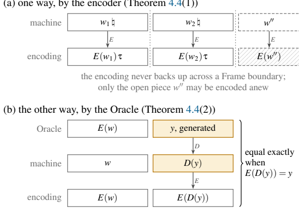
Figure 6: Frame synchronization, both ways. (a) When the encoder factorizes at \natural , the encoding of a history is the concatenation of the encodings of its pieces up to each \natural (answers and the kernel’s records alike, each ending with \tau ), followed by that of the open piece w'' . Only the open piece may be re-encoded differently as the history grows. (b) After the Oracle answers a history w (empty or ending with \natural ) with the Frame y , its own history is E(w)y , while the machine records wD(y) , whose encoding is E(w)E(D(y)) . The two are equal exactly when the Frame re-encodes to itself, and otherwise they diverge inside the Frame. Amber: what the Oracle generated.
