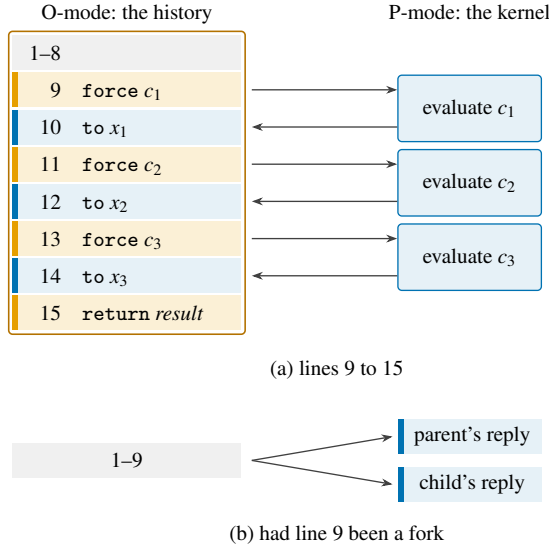
Figure 11: The history of Figure 10 read from O-mode as one program (amber: the Oracle’s answers; blue: the kernel’s replies and its work in P-mode). (a) Each call c_i forces a thunk the declaration offers. The kernel evaluates it in P-mode, and the value is returned and bound with to . The rest of the history is the continuation. (b) Had the answer at line 9 been a fork, the parent’s history and the child’s would share lines 1 to 9, each followed by its own reply.
