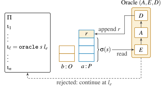
Figure 3: The O-2-PDA. The program \Pi runs on two stacks, coloured P (blue outline) and O (amber outline). The instruction \text{oracle } s l_e reads the whole content of the stack s , here a . The encoder E maps it to a query, and the decoder D maps an answer of A to a word r \in O(\sigma(s)) , which is appended to s . The word r is filled amber because the Oracle wrote it, and since it lies on a , it has colour P in the sense of Definition 2.3. When E rejects a query, the machine continues at l_e .
