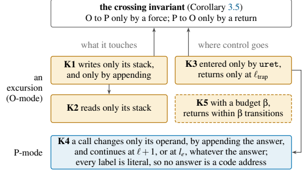
K1, K3 and K4 follow from the rules of T, and K5 from those of the budget; K2 and the crossing invariant also use the locality lemma
