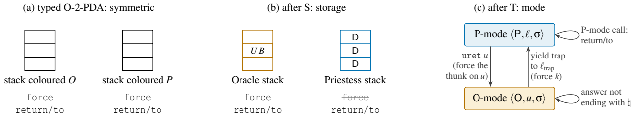
Figure 4: The two breakings. (a) The typed O-2-PDA: on every stack the Oracle instruction may be read as a force or as a return/to. (b) After S: on a Priestess stack (blue) every element has type D and the Oracle instruction is only a return/to (force struck out); on an Oracle stack (amber) content may have type UB , and both readings remain. (c) After T: \text{uret } u enters O-mode on the Oracle stack u , O-mode appends answers to u until one ends with \natural , and the yield trap continues at \ell_{\text{trap}} . P stands above O.
