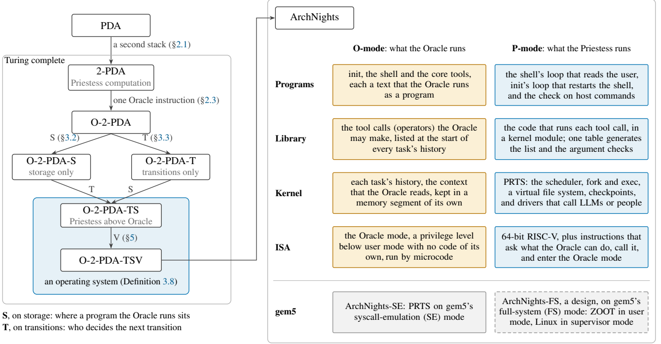
Figure 2: The construction. Left: the abstract machines from the PDA to the O-2-PDA-TSV. S and T are the two symmetry breakings, which can be taken in either order and together make a Priestess program the operating system of the tasks the Oracle runs. V realizes the O-2-PDA-TS on a von Neumann computer. Right: ArchNights, the prototype that implements the O-2-PDA-TSV on gem5, with what runs in O-mode on the Oracle side (amber) and what runs in P-mode on the Priestess side (blue). The bottom row, not split by side, holds the two realizations. ArchNights-SE runs the kernel PRTS on gem5's SE mode, and ArchNights-FS (dashed) is a design with the kernel ZOOT.
