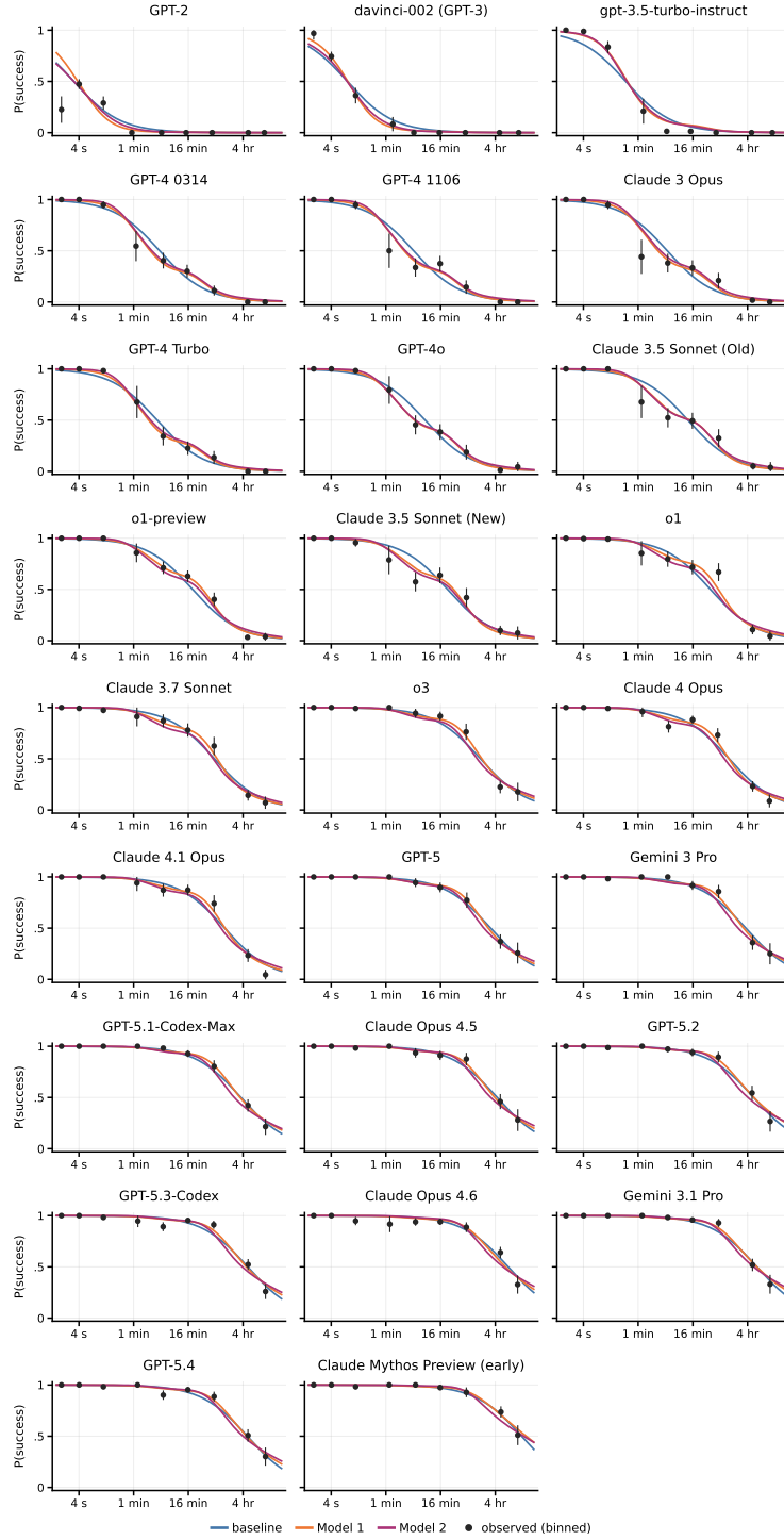
Figure 9: In-sample fitted p_j(t) against binned observed frequencies for all 26 AIs , in release order; construction as in Figure 4 (factor-4 human-time bins centered on 1 min, 4 min, 16 min, ...; points at run-weighted mean human times, 95% Wald intervals treating runs as independent). The shape misfit of the log-linear baseline is concentrated in the mid-strength AIs of the GPT-4 era; for the weakest AIs the curves differ mainly in the tail, and for the strongest the three specifications nearly coincide.
