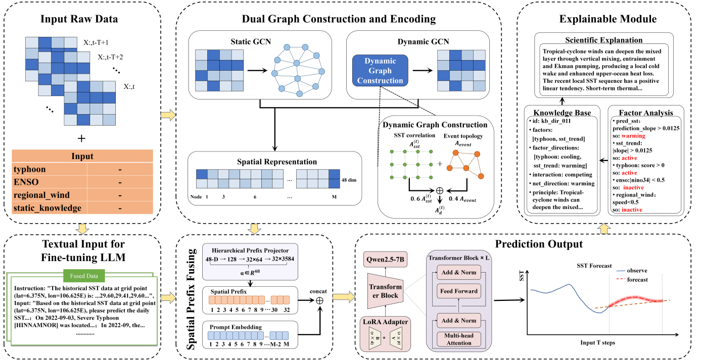
Fig. 1. Overview of the framework. At forecast origin t , target-cell SST and anomaly histories, environmental records, and static ocean knowledge form a textual condition. Regional observations construct a static geographic-climatological graph and a date-specific dynamic graph. Two GNN branches encode the target-node state, which a factorized projector maps to continuous prefix tokens for autoregressive LLM forecasting. A separate rule-based module then matches forecast trends and environmental factors with knowledge entries for source-linked post-hoc contextualization.
