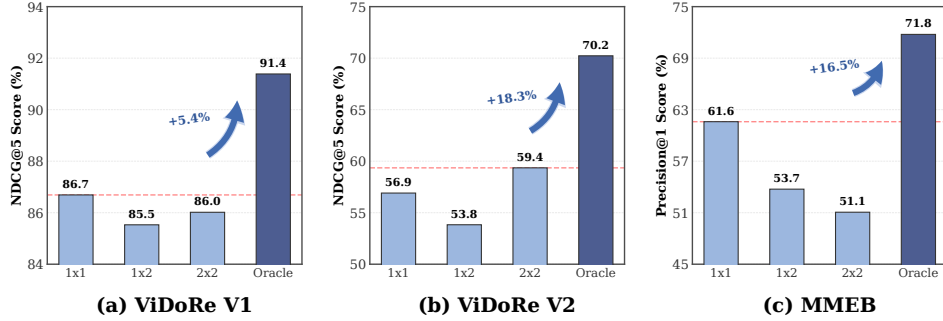
Figure 3: Single-granularity and oracle combined-selector results. ViDoRe V1/V2 use NDCG@5; MMEB uses Precision@1.
