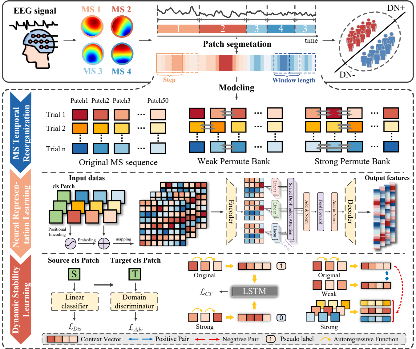
Figure 1: Overview of the proposed model framework. The model consists of four main components. (1) Microstate sequence construction. Preprocessed EEG signals are subjected to a two-step microstate clustering procedure using the k-means algorithm to obtain optimal microstate templates. These templates are then back-fitted to each data segment to generate corresponding microstate time series. (2) MS temporal reorganization. The microstate sequences are segmented into patches using sliding windows (window length = 50, step size = 50). Two shuffling strategies (weak permutation and strong permutation) are further applied to enhance the diversity of temporal patterns and improve model robustness. (3) Neural representation learning. A PatchTST architecture is employed to capture dynamic transition patterns within the microstate sequences and map them into high-dimensional representations. A dedicated CLS patch is introduced to facilitate the integration of local segment-level characteristics and global sequence-level structure. (4) Dynamic stability learning. The model is jointly optimized using multiple objectives, including a disease-specific loss, domain adversarial loss, consistency loss, and contrastive learning loss. This joint optimization enables the model to anchor disease-relevant pathological microstate transition patterns associated with NSSI, thereby simplifying subtle differences between patient subgroups.
