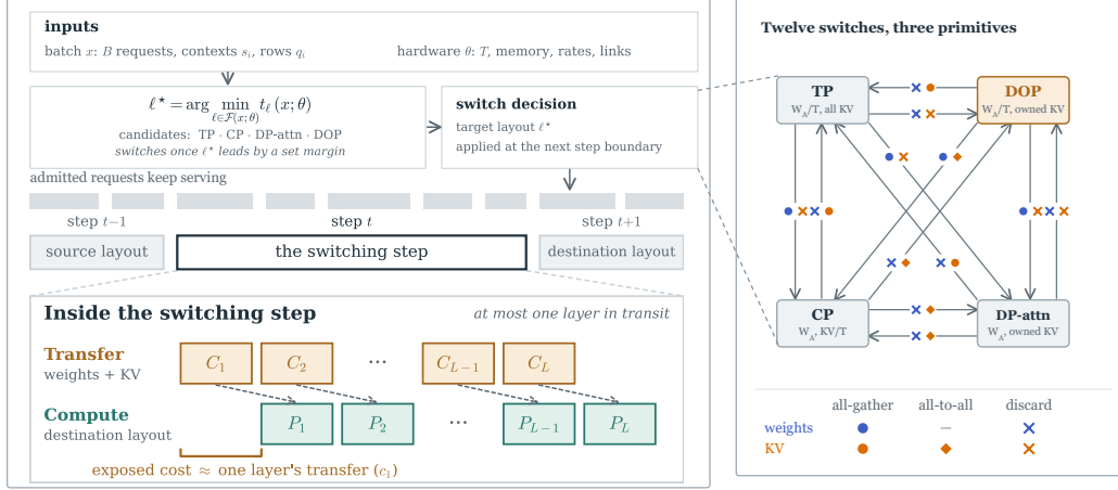
Figure 3: SPLASH. Left: the scheduler runs the fastest feasible layout and switches once another leads by a set margin (§ 4.2). Admitted requests keep serving: layer i 's transfer ( C_i ) overlaps layer i - 1 's computation ( P_{i-1} ), exposing about one layer's transfer ( c_1 ) with at most one layer in transit. Right: the A_4^2 = 12 directed switches; arrows show the primitives for weights (blue) and KV (orange). A discard keeps what the destination needs and frees the rest at zero network cost.
