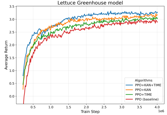
Figure 3: Ablation study on policy representation enhancements. Training performance comparison between baseline PPO, PPO with cyclic time features, and PPO with KAN-based policy networks. All methods are trained without RCPO constraint regulation.
