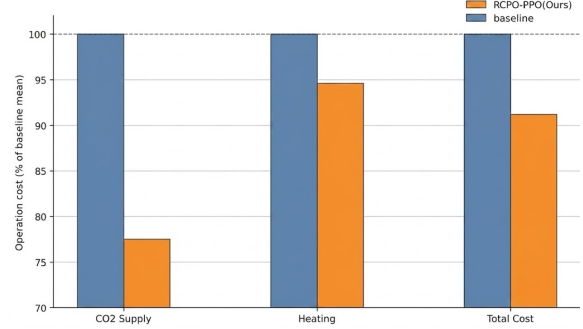
Figure 5: Normalized cumulative operation costs associated with heating and CO 2 input achieved by the proposed RCPO-PPO controller relative to the baseline PPO controller. The baseline PPO result is normalized to 100%.
