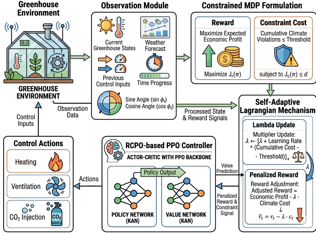
Figure 1: Framework of the proposed KAN-based safe reinforcement learning greenhouse climate control system.
