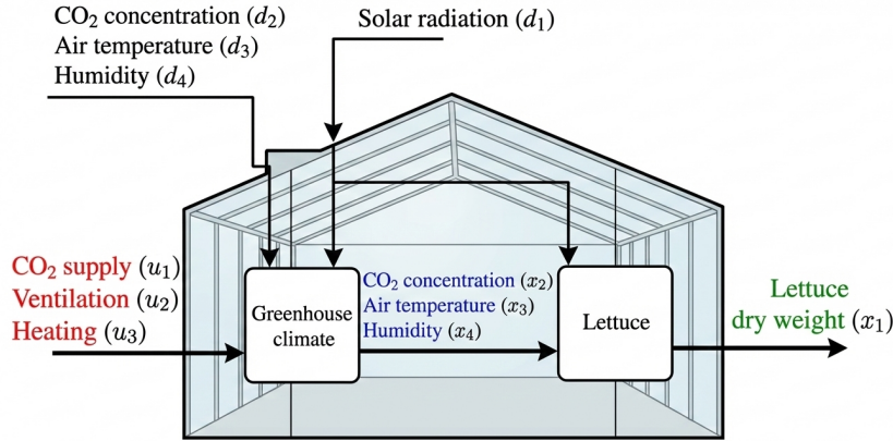
Figure 2: Greenhouse-crop system dynamic relationship diagram.
