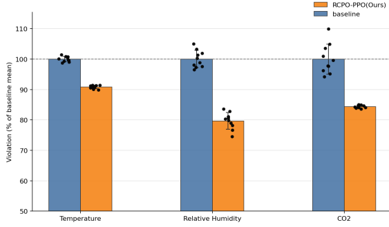
Figure 4: Normalized cumulative climate constraint violations for different climate variables achieved by the proposed RCPO-PPO controller relative to the baseline PPO controller. The baseline PPO result is normalized to 100%.
