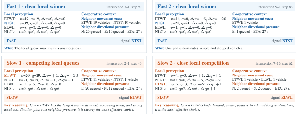
Figure 3: Case study on adaptive reasoning.
