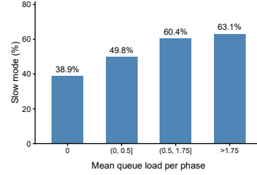
Figure 2: Slow-mode ratio across local queue-load groups.
