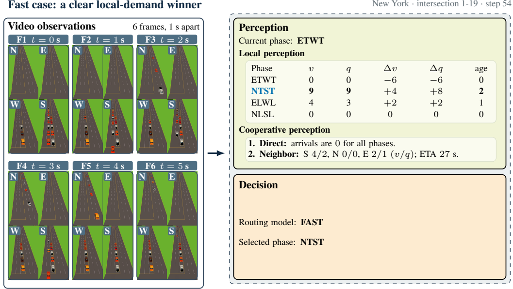
Figure 6: Fast case. A clear local-demand winner leads to fast routing.
