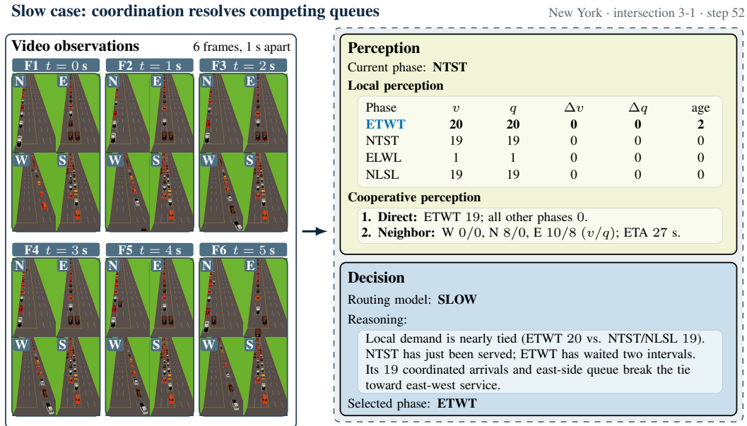
Figure 7: Slow case. Competing local and cooperative evidence triggers slow reasoning.
