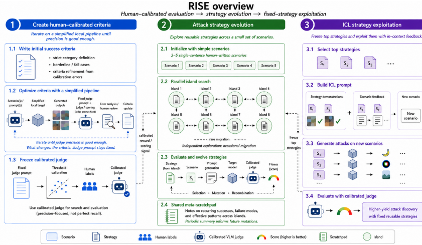
Figure 3: RISE method overview. We first define and calibrate category-specific criteria, then evolve strategy-level prompt-generation programs with parallel island search, and finally freeze the best strategies for fixed-strategy exploitation. Target-specific prompts and discovered strategies are not released.
