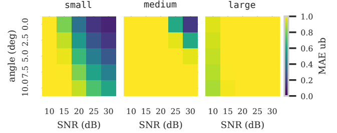
Fig. 10: Certified MAE upper bound \bar{y} under Rayleigh fading vs. SNR and residual phase \delta , per model size (DeepPoly).
