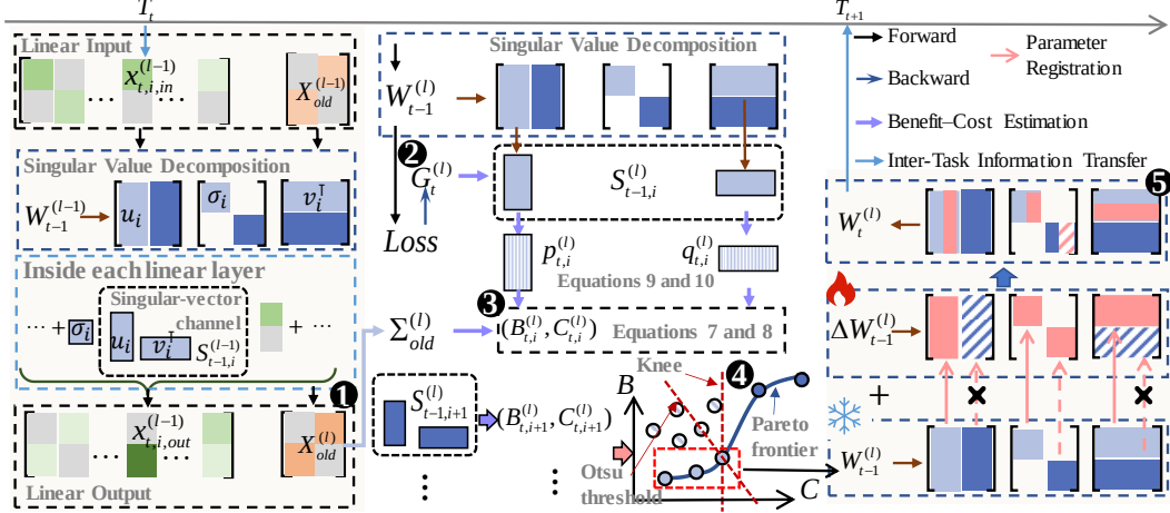
Figure 2: Overview of SVC. SVC ① collects reference activation statistics from a publicly available, unlabeled general-domain reference corpus. It then ② computes layer-wise average gradients from current-task data. From these quantities, SVC ③ estimates each singular-vector channel’s local adaptation benefit and forgetting cost. SVC next ④ selects trainable channels through knee-based cost screening, Pareto-frontier filtering, and Otsu thresholding. Finally, SVC ⑤ updates all singular values while updating singular vectors only in selected channels. Post-training, SVC merges the learned increments into the model weights.
