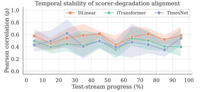
Figure 3: Pearson correlation between s_t and future degradation g_t^{\text{online}} across the test stream. Lines show means across datasets and seeds; shading denotes the interquartile range.
