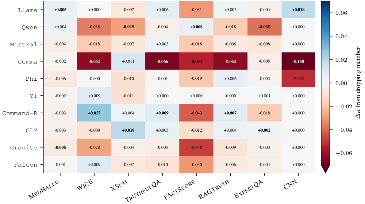
FIG. 5. Leave-one-out change in stacked \kappa from dropping each member ( \Delta = stacked without member - full stacked): red marks a load-bearing member, whose removal costs the panel, blue one the panel can spare. Every cell carries its value, and each column’s extremes are set in bold. The colour scale is clipped at \pm 0.07 for legibility, Gemma on CNN at -0.158 being off-scale.
