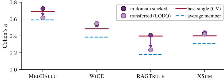
FIG. 8. Leave-one-dataset-out transfer on the four core grounded sets: in-domain stacked and transferred (LODO), against the CV-best single judge and the average member per dataset.
