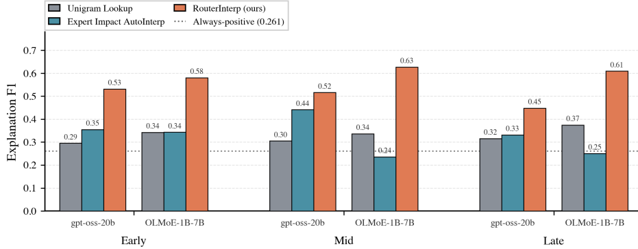
Figure 4. Leveraging the SSH, RouterInterp generates expert explanations from examples where SAE features and experts are jointly active. It outperforms both a method based on token-statistics (Jiang et al., 2024; Zoph et al., 2022) and Expert Impact AutoInterp (Herbst et al., 2026), which generates explanations from activating windows ranked by expert impact on the residual stream, at every model depth ( \sim 65\% / \sim 76\% mean F1 over Unigram Lookup on gpt-oss-20b / OLMoE-1B-7B; \sim 28\% over Expert Impact AutoInterp on gpt-oss-20b). Shown for layers 4, 16, 20 of gpt-oss-20b and layers 3, 11, 15 of OLMoE-1B-7B.
