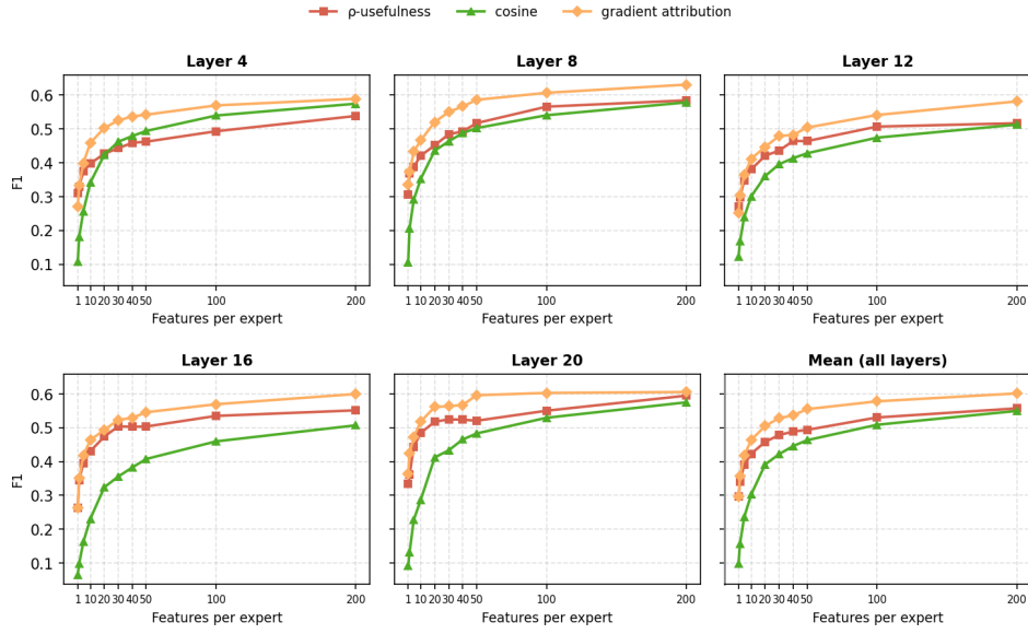
Figure 5. Gradient-based attribution is the strongest feature-selection criterion across five layers of gpt-oss-20b and every feature set size n . For each feature selection method, we select the top- n features per expert and train a linear probe to predict routing to an expert using only these features’ activations. The mean F1 across layers improves only gradually beyond \sim 50 features.
