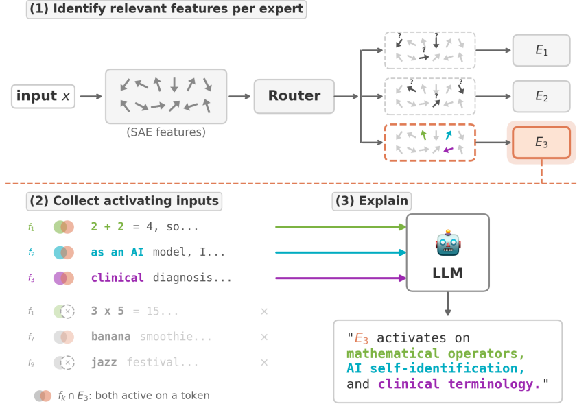
Figure 3. RouterInterp explains routing decisions as a combination of interpretable features. Sparse autoencoder (SAE) latents, sparse feature representations extracted from model activations, pick out directions in activation space that correspond to interpretable features. RouterInterp identifies SAE latents that are most predictive of routing, collects inputs where these features and the expert are jointly active, and explains the expert in natural language. While no single monosemantic concept captures an expert’s behaviour, aggregating multiple features makes routing understandable.
