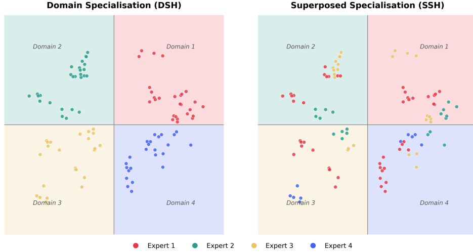
Figure 1. Illustration of two alternative hypotheses for the expert specialisation in MoE models. Left: Under the Domain Specialisation Hypothesis, examples (points) from the same semantic domain (coloured region) are routed to the same expert, so each expert specialises in a single coherent domain. Right: Under the Superposed Specialisation Hypothesis, examples routed to the same expert are scattered across different domains. Here the clusters of adjacent points routed to the same expert represent micro-domains (fine-grained features of a particular domain) and each expert specialises in a disjoint union of them. We suggest that the SSH is a more accurate description of expert specialisation in practice.
