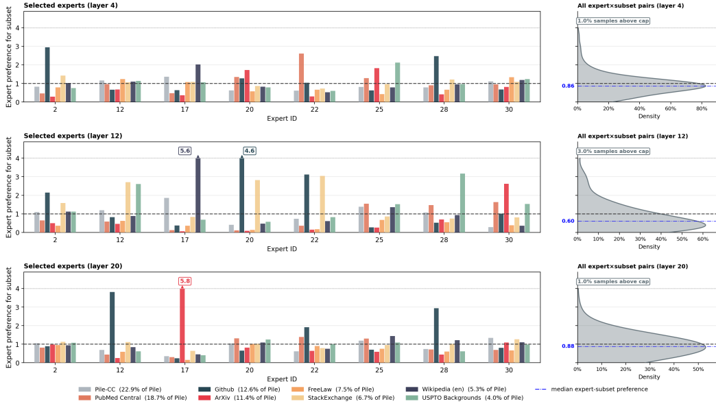
Figure 7. Expert routing distributions across Pile domains provide evidence against macro-domain DSH and are consistent with SSH. Adapting the Mixtral analysis of Jiang et al. (2024) on gpt-oss-20b, we plot how often an expert’s routed tokens come from a subset, relative to this subset’s fraction of the corpus (the expert routing preference ). We show routing preferences for randomly selected experts across 16 subsets (left) and their density over all expert–subset pairs (right), at an early (layer 4), a middle (layer 12), and a late (layer 20) layer. The densities are tightly concentrated at the corpus rate (dashed line at 1). If expert domains coincided with Pile subsets, preferences would instead spread far from 1: near zero for most pairs, and at many times the corpus rate for a few dedicated specialists. Values above 4.0 are capped for better readability.
