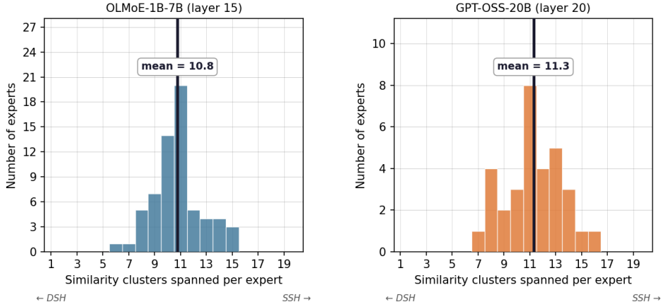
Figure 2. Each expert covers a semantically diverse range of micro-domains: the latents that best predict its activation are spread across many distinct semantic clusters. For each expert we take its top n=20 predictive SAE latents \mathbb{F}_i and cluster them semantically by their explanations. The DSH predicts one shared cluster; the SSH predicts a separate cluster per latent. We observe that experts’ latents are grouped into far more than one cluster: 10.8 clusters on average for OLMoE-1B-7B (layer 15) and 11.3 for gpt-oss-20b (layer 20).
