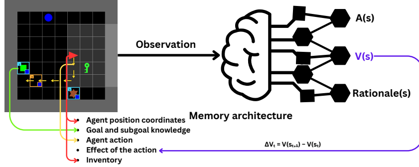
Figure 1: A flow diagram of how STRAT gets the required labels without human intervention.
