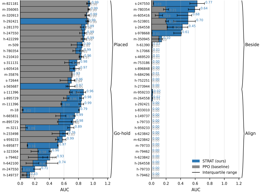
Figure 2: Comparison of STRAT and PPO across 60 tasks. The bars represents mean normalized AUC of the learning curve. The whiskers are the interquartile range for 10 seeds. The numbers represent the mean final returns.
