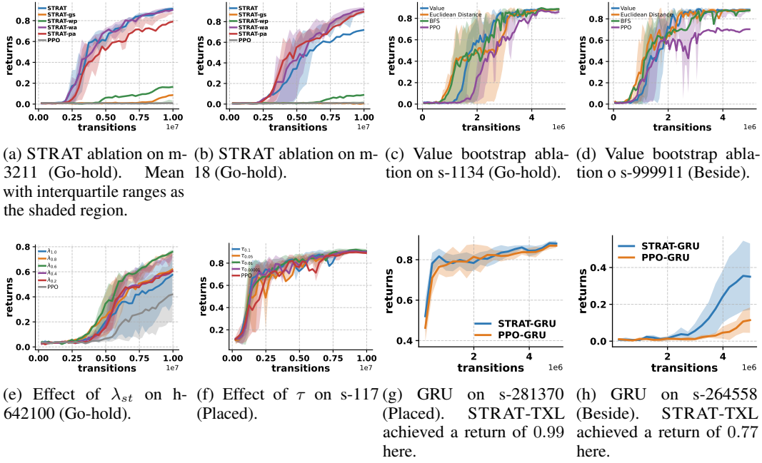
Figure 3: Ablations, \lambda_{st} and \tau sweeps, and GRU learning curves.
