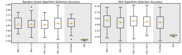
Figure 7: Comparative performance of cut-based features (WLC-n/WLC-ne) against fzn2feat and the majority classifier (MC) baseline. Results on the left are obtained by training RF models, while those on the right are obtained by training MLPs.
