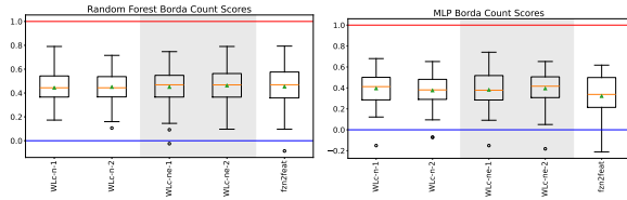
Figure 5: Comparative performance of cut-based features (WLC-n/WLC-ne) against the fzn2feat baseline for the Borda count maximization task. Scores are normalised relative to the Single Best Solver and Virtual Best Solver. Results on the left are obtained by training RF models, while those on the right are obtained by training MLPs.
