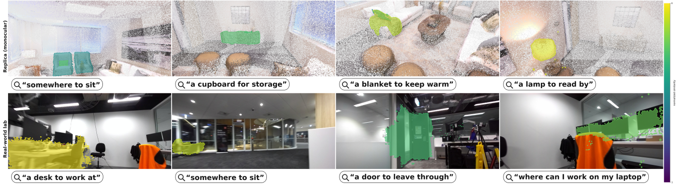
Fig. 3. Open-vocabulary queries resolve to the correct object instances on both the benchmark map and a real building. Each panel shows a free-form language query (search bar) and the instances VOIM retrieves, colored by normalized query–instance similarity (per-scene). Top : the fully monocular Replica room0 map (the same reconstruction scored in Table I), rendered as a point cloud. Bottom : the real-world lab 3D map (sensor RGB-D + on-board VIO); retrieval and instance identity come from this map, with the resulting 3D instances reprojected into the 2D capture frames for display. Queries are resolved by cosine similarity between the phrase embedding and each instance’s aggregated vision–language embedding, so compositional phrases (“a cupboard for storage”, “where can I work on my laptop”) retrieve the semantically appropriate objects.
